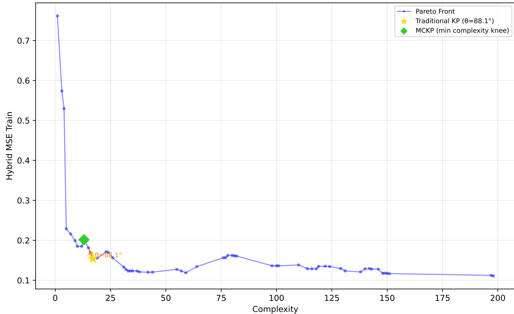
1096_FacultySalaries - Run 28 - SVP - Hybrid MSE Train \lambda_1=1.00, \lambda_2=0.00, \lambda_3=0.00 | Difficulty: 0.51 | Method: mckp
