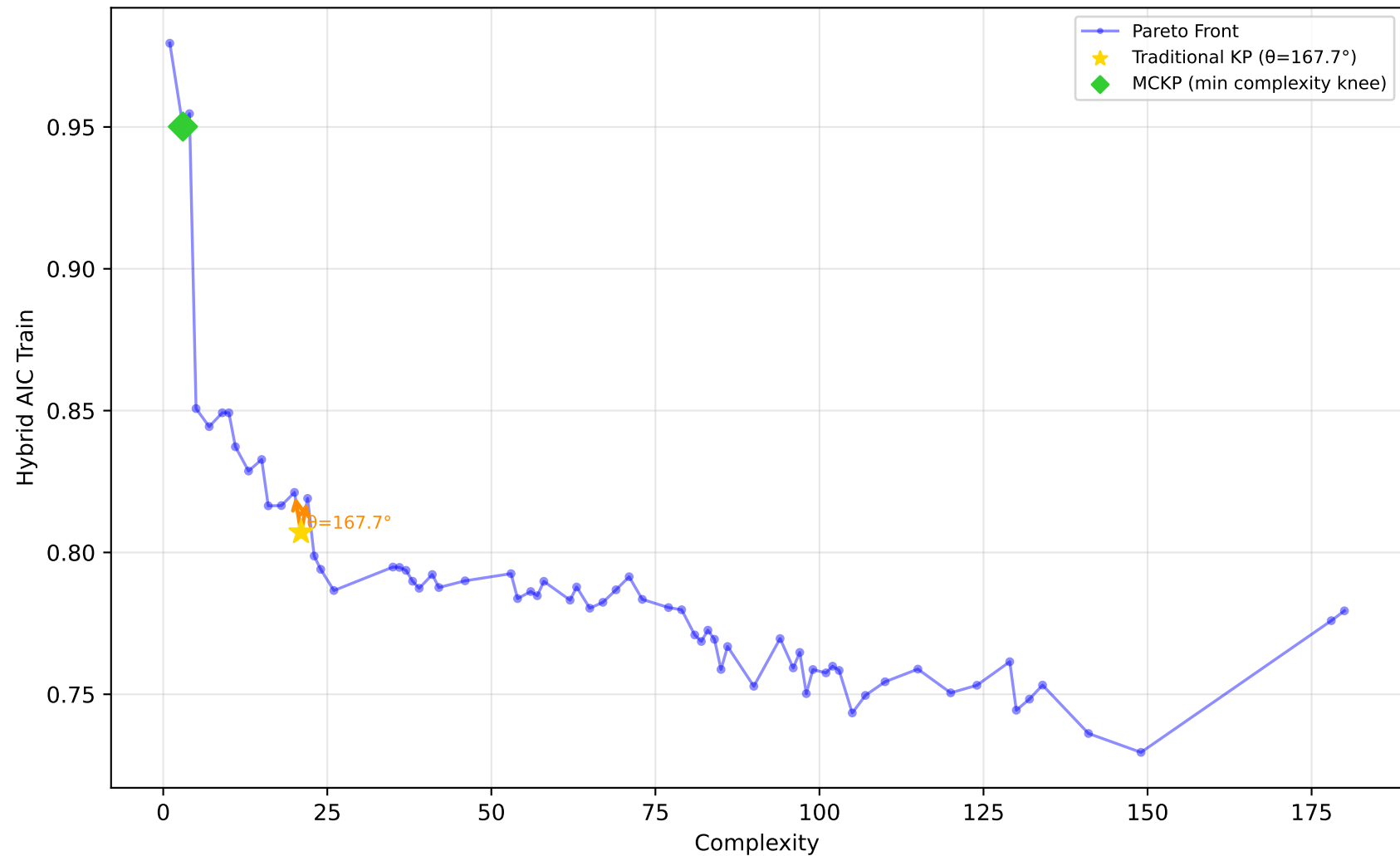
1096_FacultySalaries - Run 29 - MVP - Hybrid AIC Train \lambda_1=0.10, \lambda_2=0.00, \lambda_3=0.00 | Difficulty: 0.37 | Method: mckp
