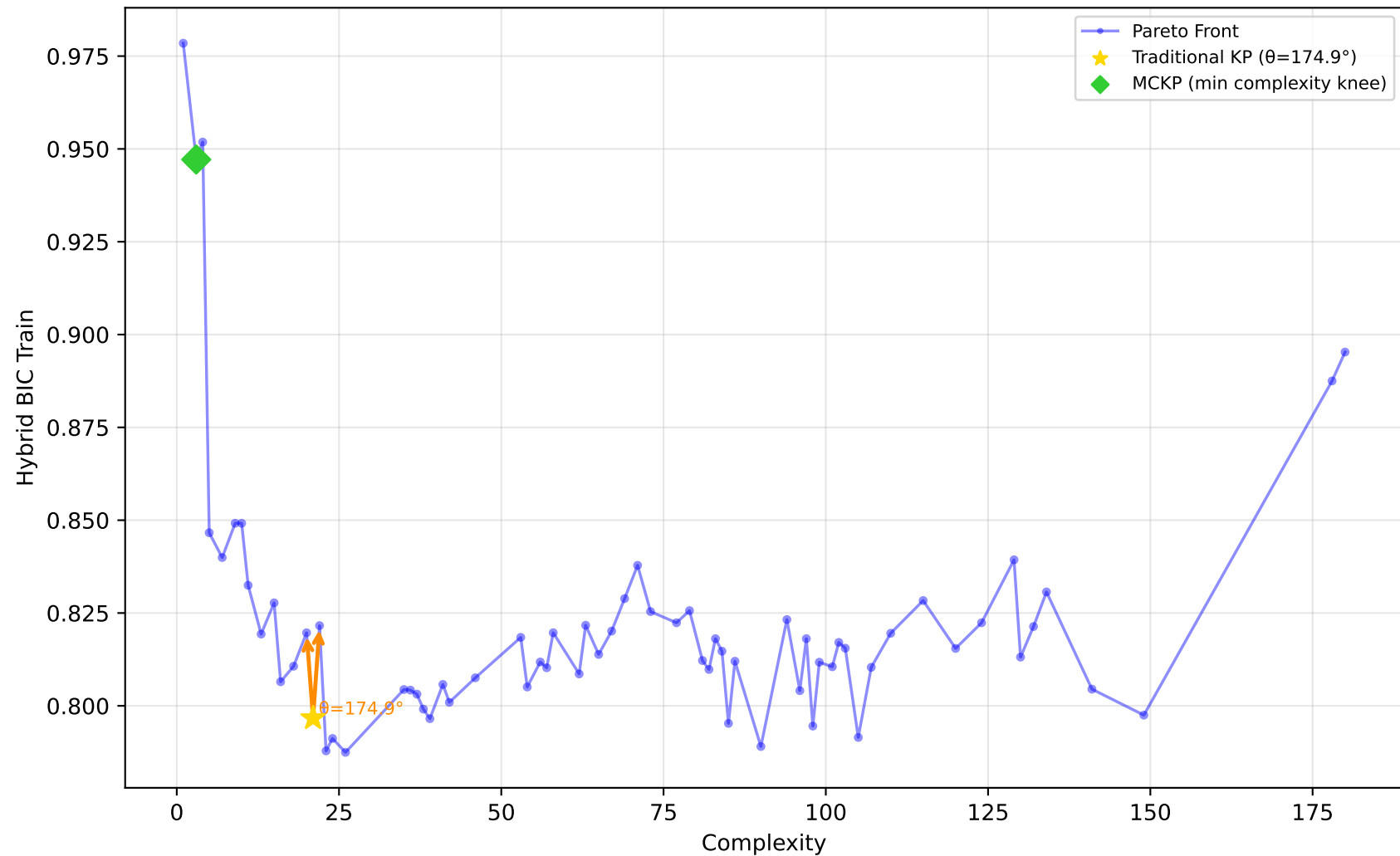
1096_FacultySalaries - Run 29 - MVP - Hybrid BIC Train \lambda_1=0.10 , \lambda_2=0.00 , \lambda_3=0.00 | Difficulty: 0.37 | Method: mckp
