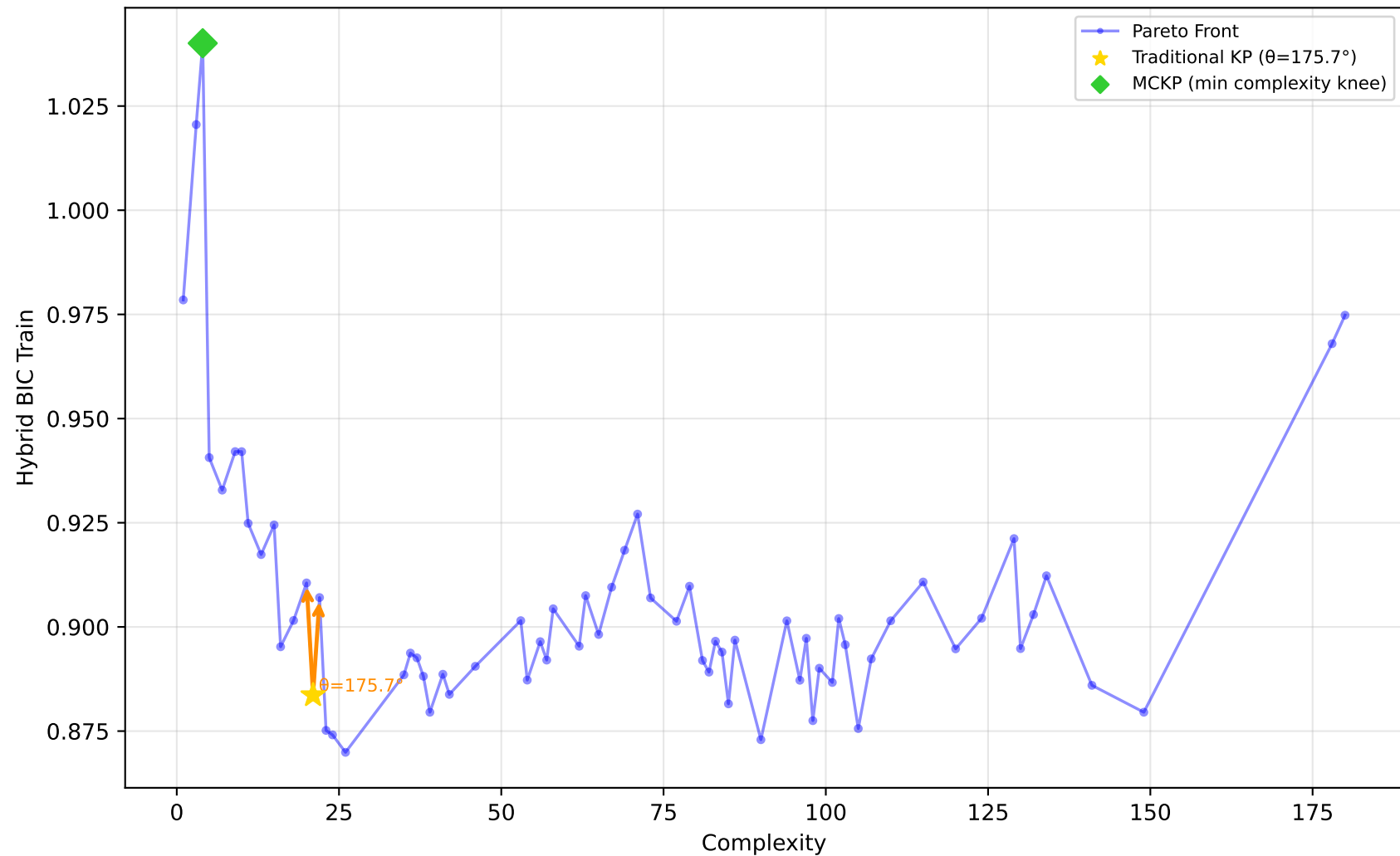
1096_FacultySalaries - Run 29 - MVP - Hybrid BIC Train \lambda_1=1.00, \lambda_2=0.00, \lambda_3=0.00 | Difficulty: 0.37 | Method: mckp
