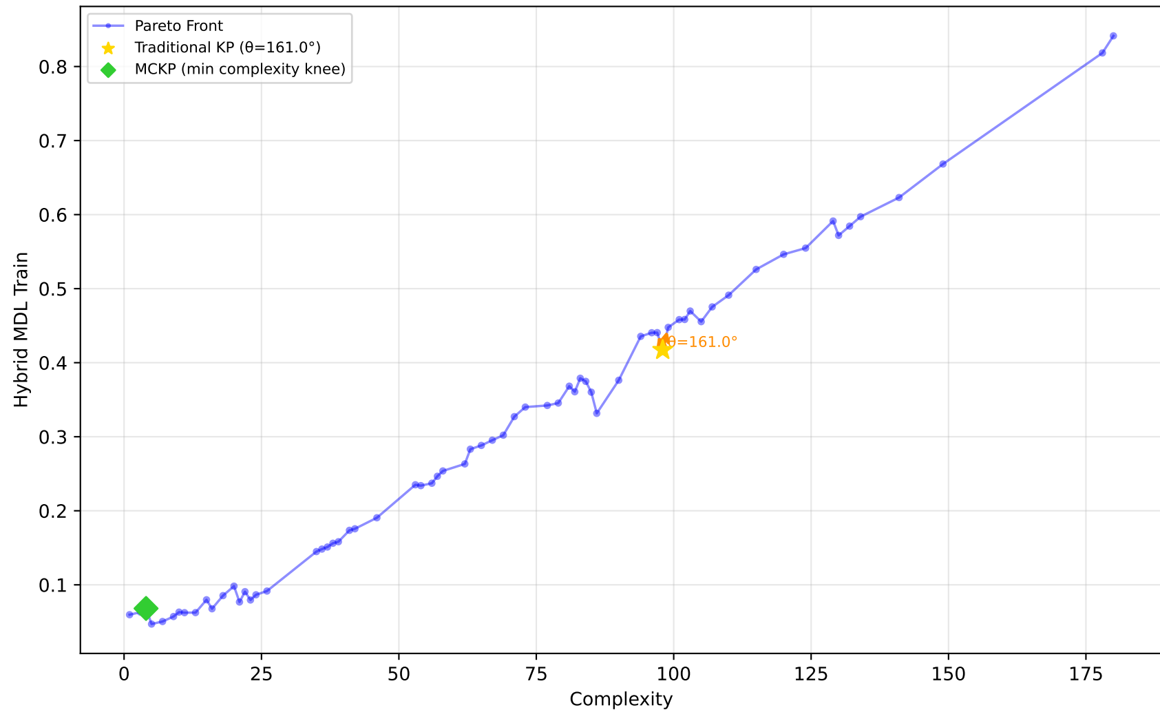
1096_FacultySalaries - Run 29 - MVP - Hybrid MDL Train \lambda_1=0.10, \lambda_2=0.00, \lambda_3=0.00 | Difficulty: 0.37 | Method: mckp
