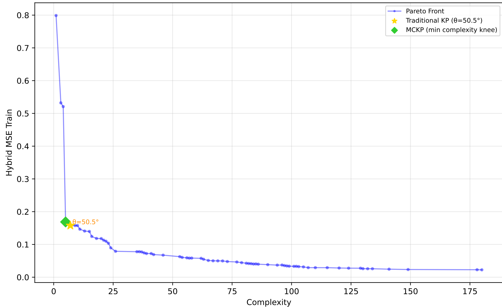
1096_FacultySalaries - Run 29 - MVP - Hybrid MSE Train \lambda_1=0.10 , \lambda_2=0.00 , \lambda_3=0.00 | Difficulty: 0.37 | Method: mckp
