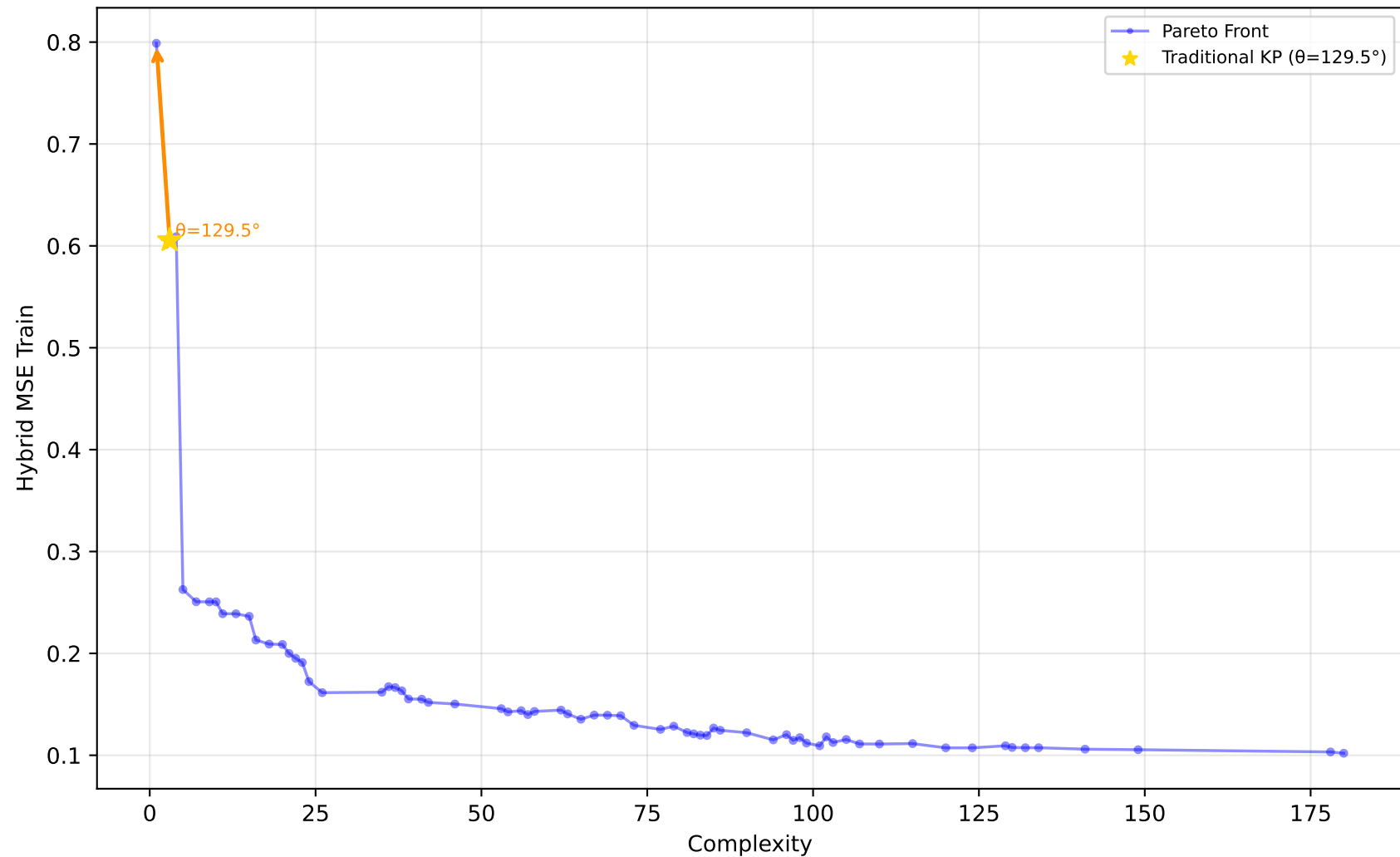
1096_FacultySalaries - Run 29 - MVP - Hybrid MSE Train \lambda_1=1.00 , \lambda_2=0.00 , \lambda_3=0.00 | Difficulty: 0.37 | Method: mckp
