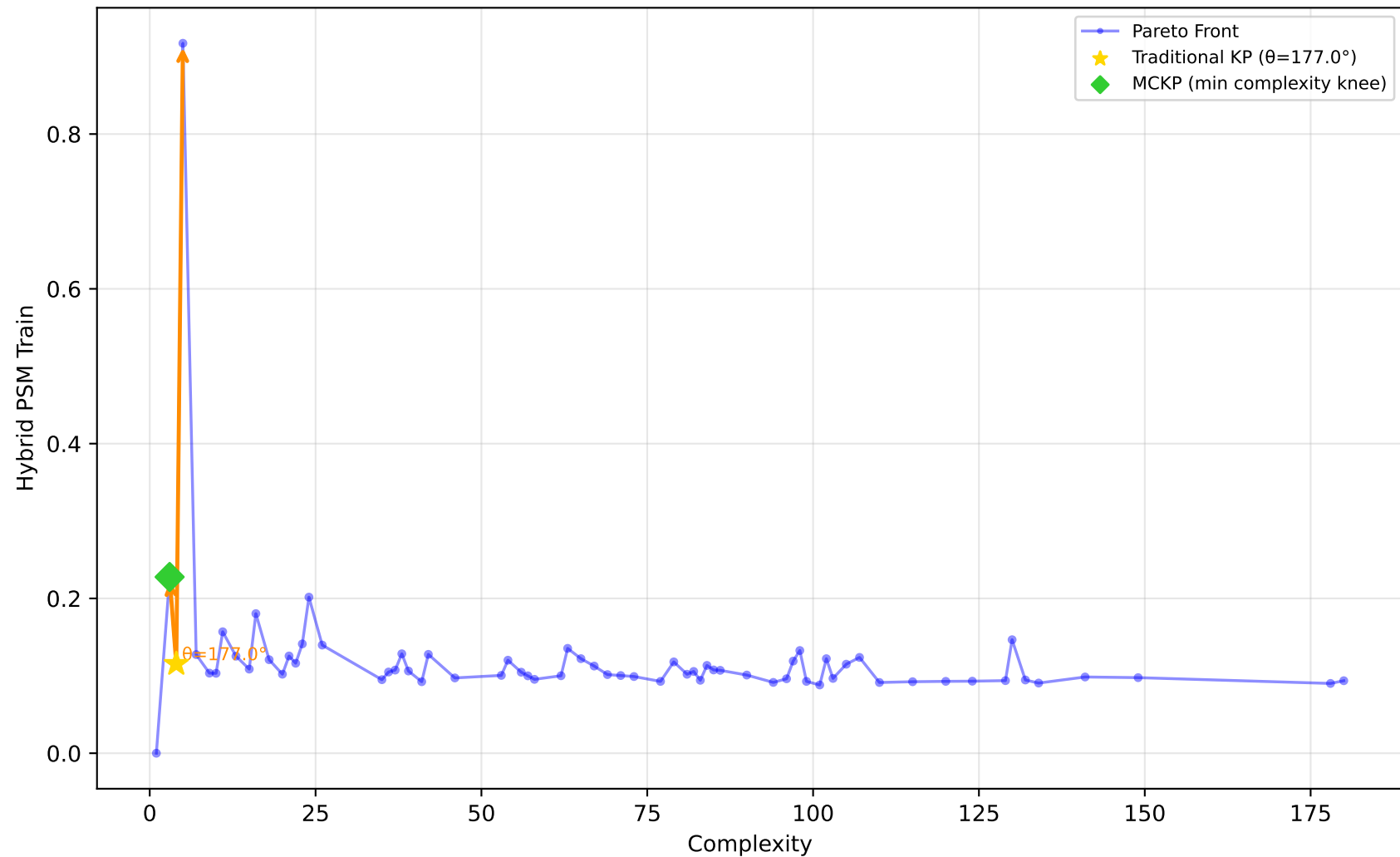
1096_FacultySalaries - Run 29 - MVP - Hybrid PSM Train \lambda_1=1.00 , \lambda_2=0.00 , \lambda_3=0.00 | Difficulty: 0.37 | Method: mckp
