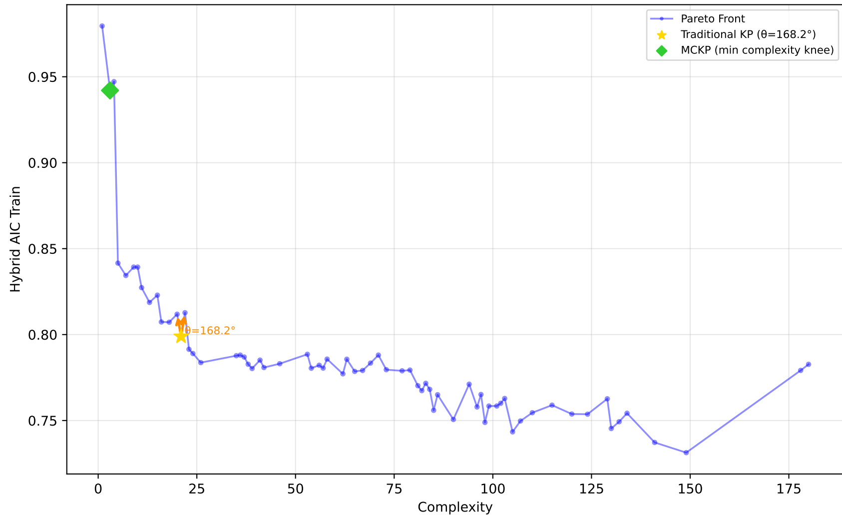
1096_FacultySalaries - Run 29 - SVP - Hybrid AIC Train \lambda_1=0.00, \lambda_2=0.90, \lambda_3=0.00 | Difficulty: 0.37 | Method: mckp
