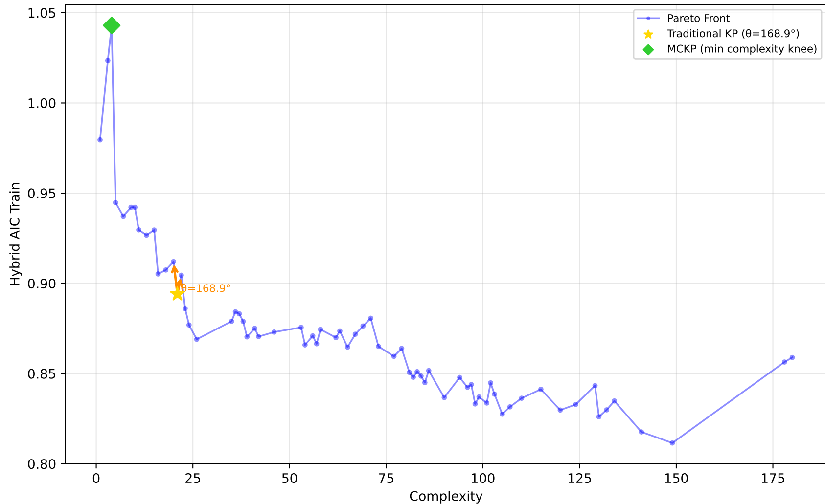
1096_FacultySalaries - Run 29 - SVP - Hybrid AIC Train \lambda_1=1.00, \lambda_2=0.00, \lambda_3=0.00 | Difficulty: 0.37 | Method: mckp
