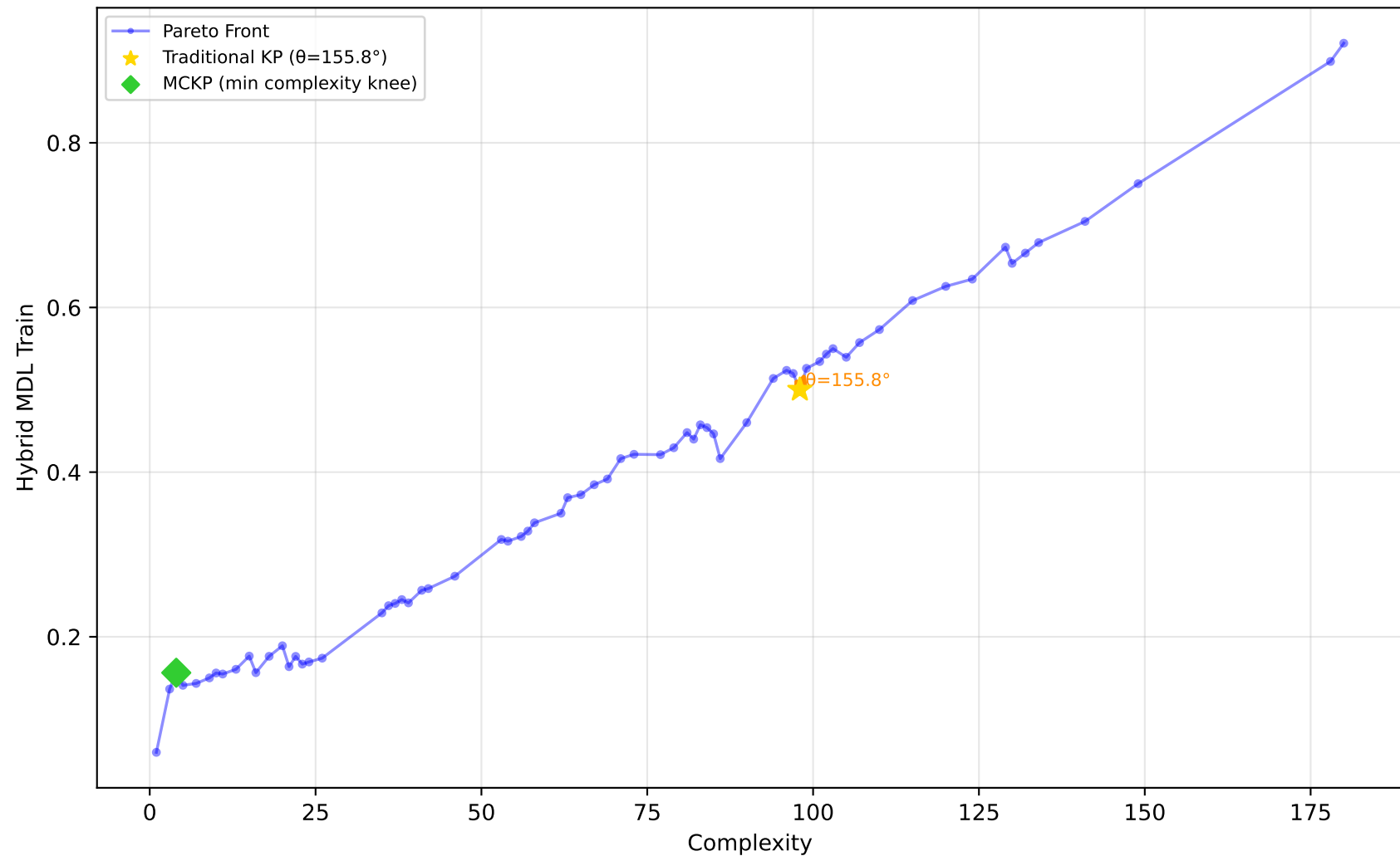
1096_FacultySalaries - Run 29 - SVP - Hybrid MDL Train \lambda_1=1.00, \lambda_2=0.00, \lambda_3=0.00 | Difficulty: 0.37 | Method: mckp
