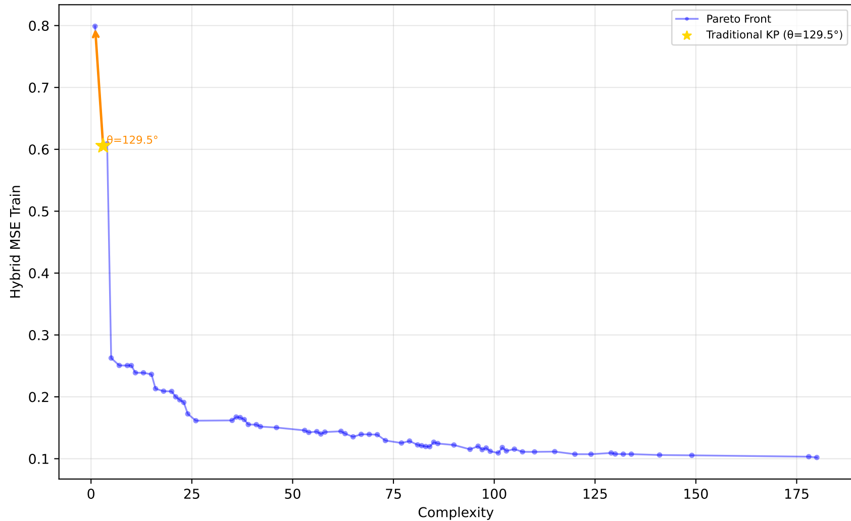
1096_FacultySalaries - Run 29 - SVP - Hybrid MSE Train \lambda_1=1.00, \lambda_2=0.00, \lambda_3=0.00 | Difficulty: 0.37 | Method: mckp
