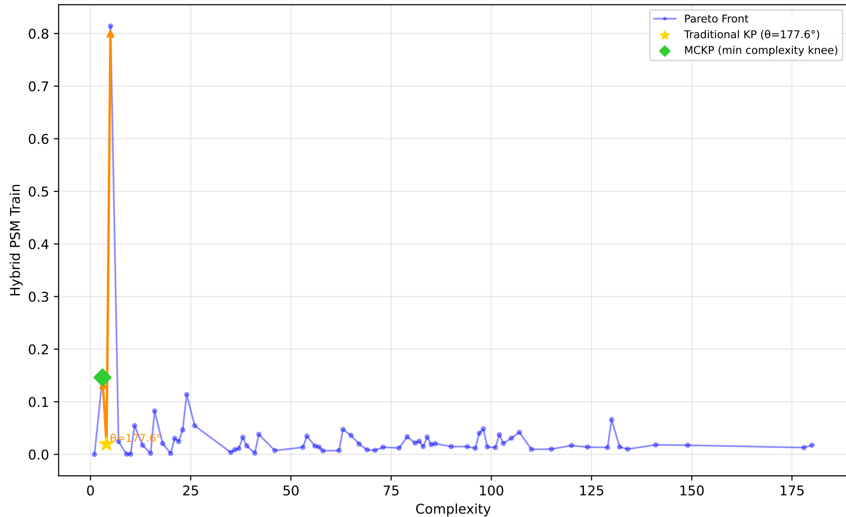
1096_FacultySalaries - Run 29 - SVP - Hybrid PSM Train \lambda_1=0.00 , \lambda_2=0.90 , \lambda_3=0.00 | Difficulty: 0.37 | Method: mckp
