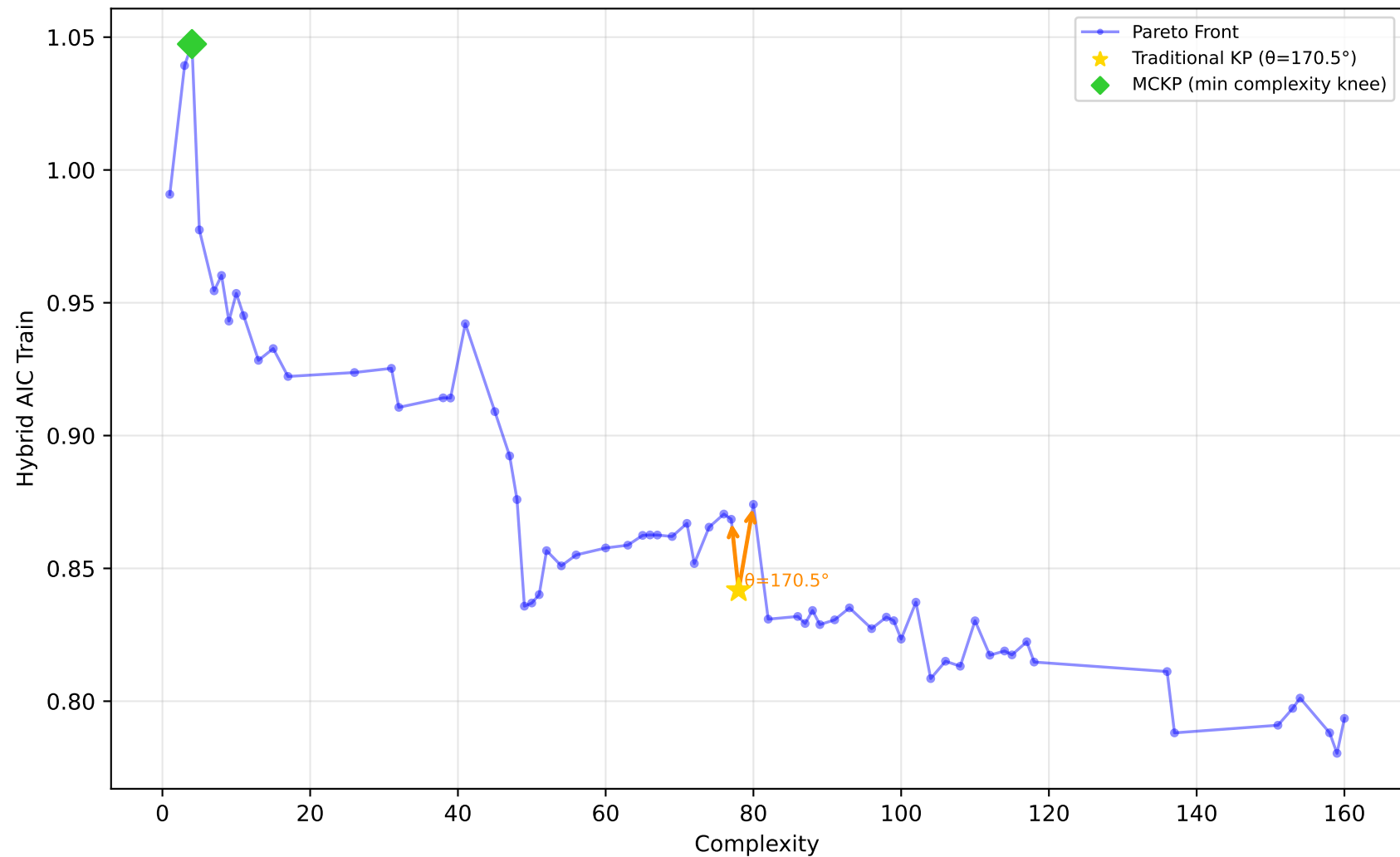
1096_FacultySalaries - Run 2 - MVP - Hybrid AIC Train \lambda_1=1.00, \lambda_2=0.00, \lambda_3=0.00 | Difficulty: 0.52 | Method: mckp
