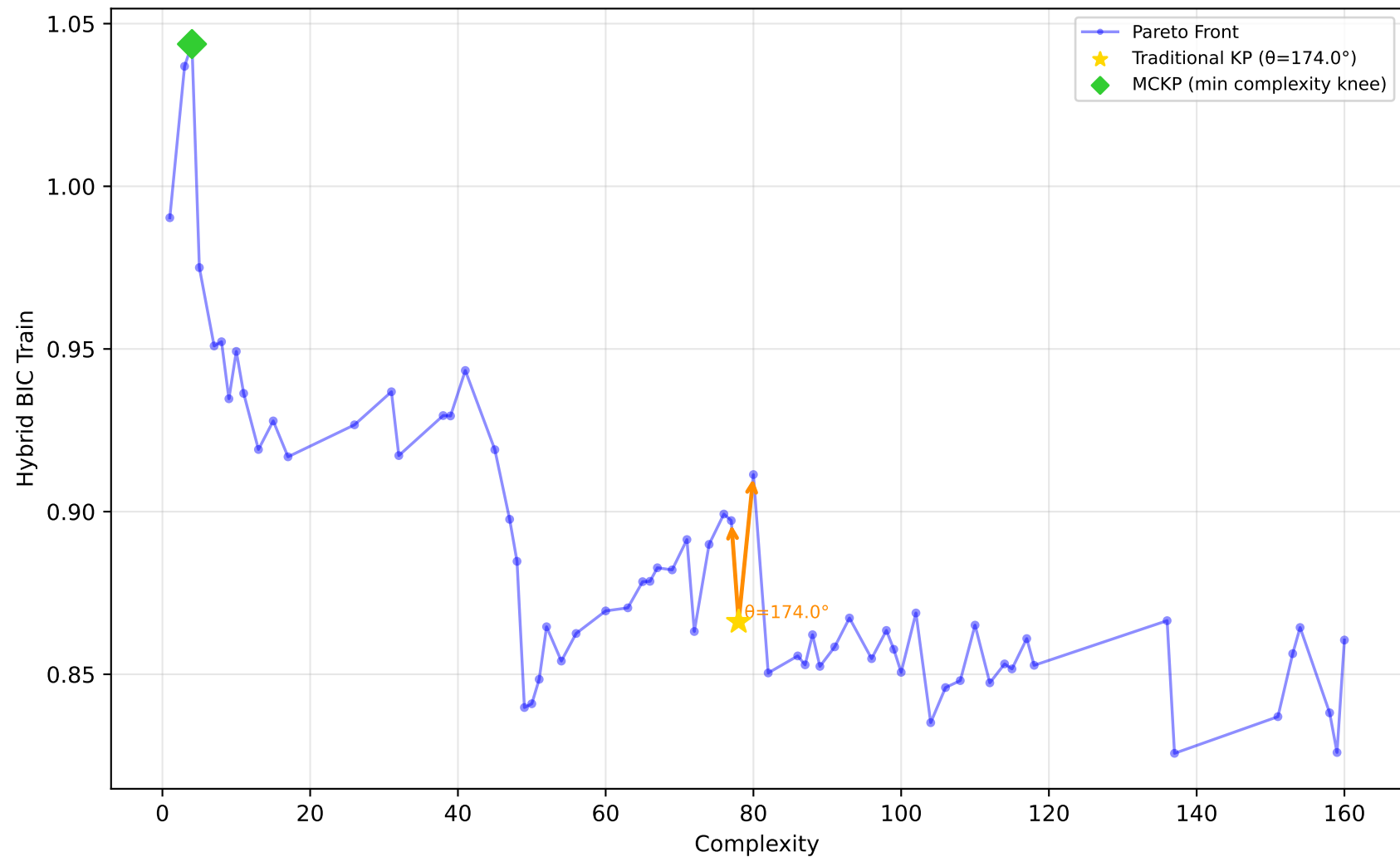
1096_FacultySalaries - Run 2 - MVP - Hybrid BIC Train \lambda_1=1.00, \lambda_2=0.00, \lambda_3=0.00 | Difficulty: 0.52 | Method: mckp
