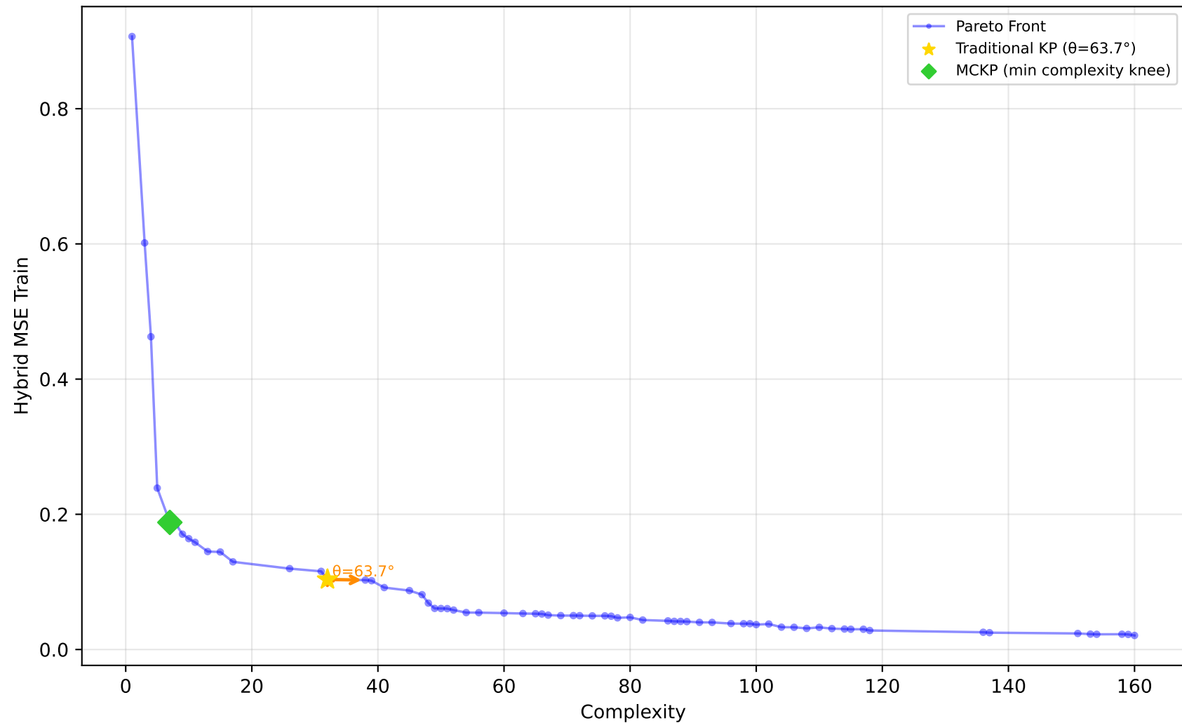
1096_FacultySalaries - Run 2 - MVP - Hybrid MSE Train \lambda_1=0.10, \lambda_2=0.00, \lambda_3=0.00 | Difficulty: 0.52 | Method: mckp
