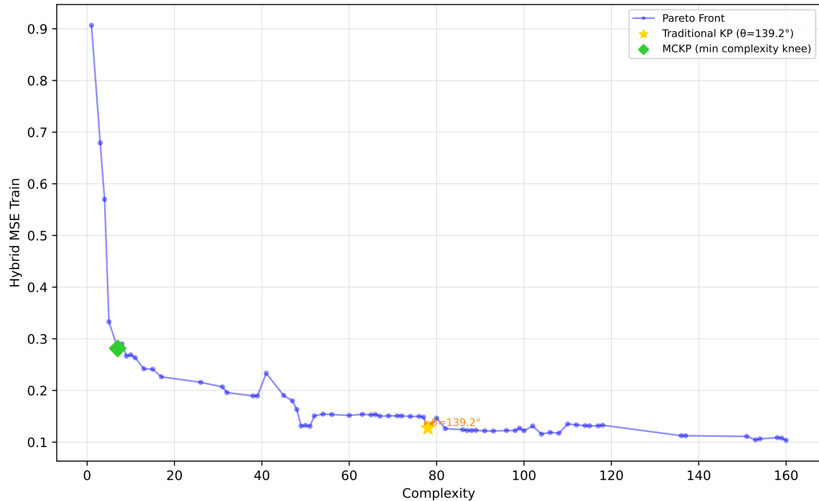
1096_FacultySalaries - Run 2 - MVP - Hybrid MSE Train \lambda_1=1.00, \lambda_2=0.00, \lambda_3=0.00 | Difficulty: 0.52 | Method: mckp
