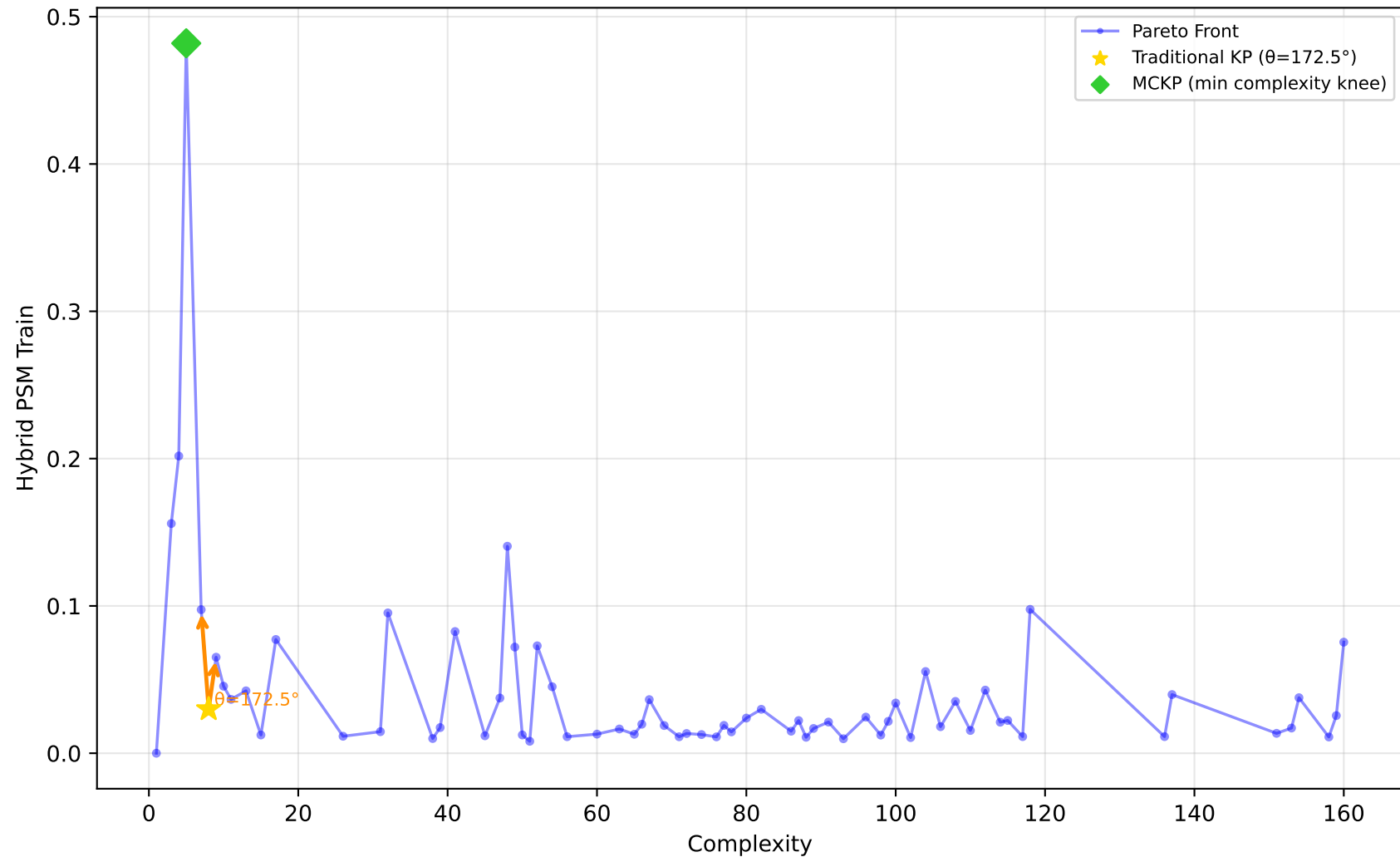
1096_FacultySalaries - Run 2 - MVP - Hybrid PSM Train \lambda_1=0.10, \lambda_2=0.00, \lambda_3=0.00 | Difficulty: 0.52 | Method: mckp
