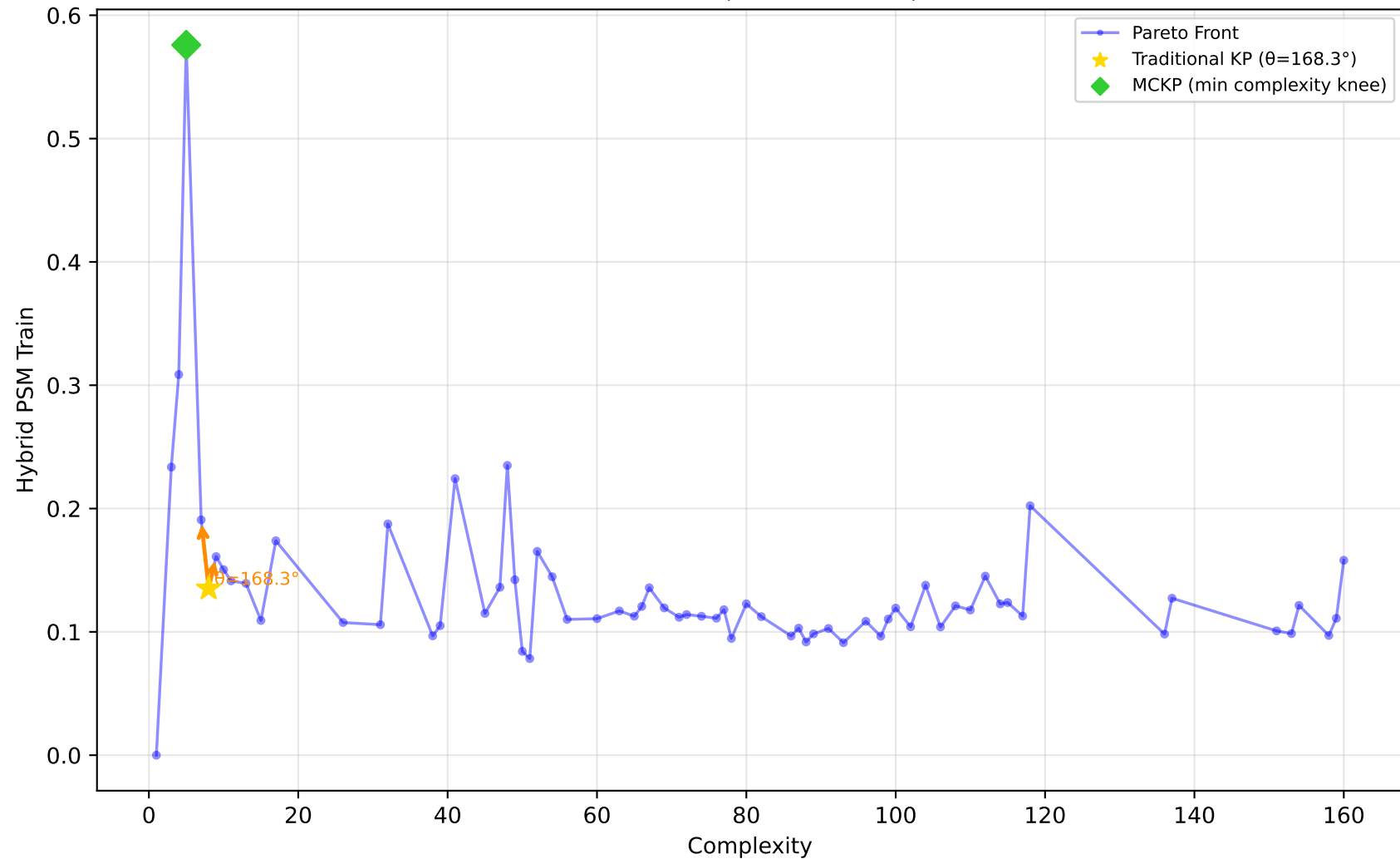
1096_FacultySalaries - Run 2 - MVP - Hybrid PSM Train \lambda_1=1.00, \lambda_2=0.00, \lambda_3=0.00 | Difficulty: 0.52 | Method: mckp
