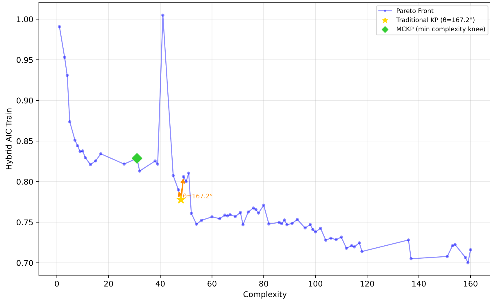
1096_FacultySalaries - Run 2 - SVP - Hybrid AIC Train \lambda_1=0.00, \lambda_2=0.90, \lambda_3=0.00 | Difficulty: 0.52 | Method: mckp
