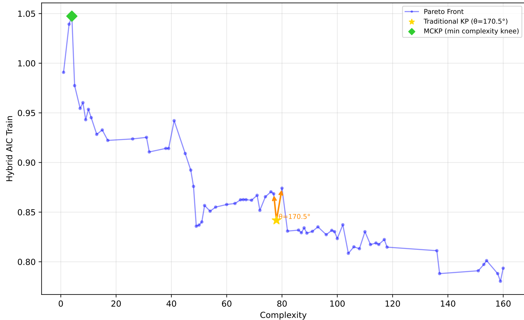
1096_FacultySalaries - Run 2 - SVP - Hybrid AIC Train \lambda_1=1.00, \lambda_2=0.00, \lambda_3=0.00 | Difficulty: 0.52 | Method: mckp
