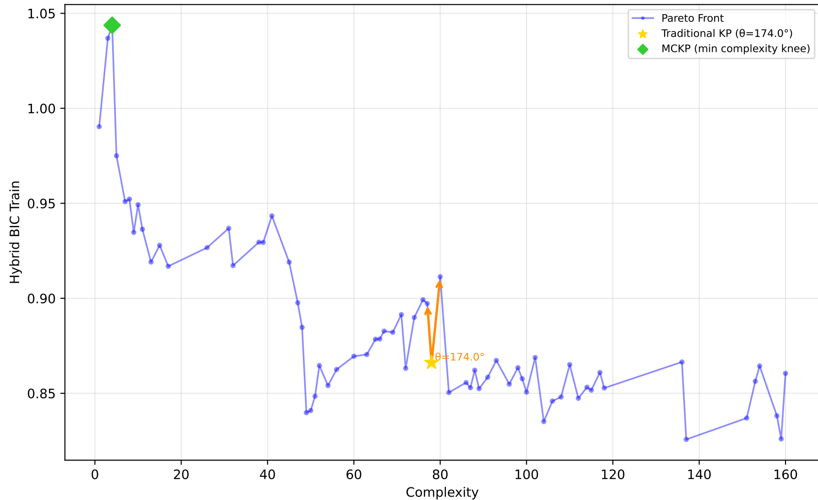
1096_FacultySalaries - Run 2 - SVP - Hybrid BIC Train \lambda_1=1.00, \lambda_2=0.00, \lambda_3=0.00 | Difficulty: 0.52 | Method: mckp
