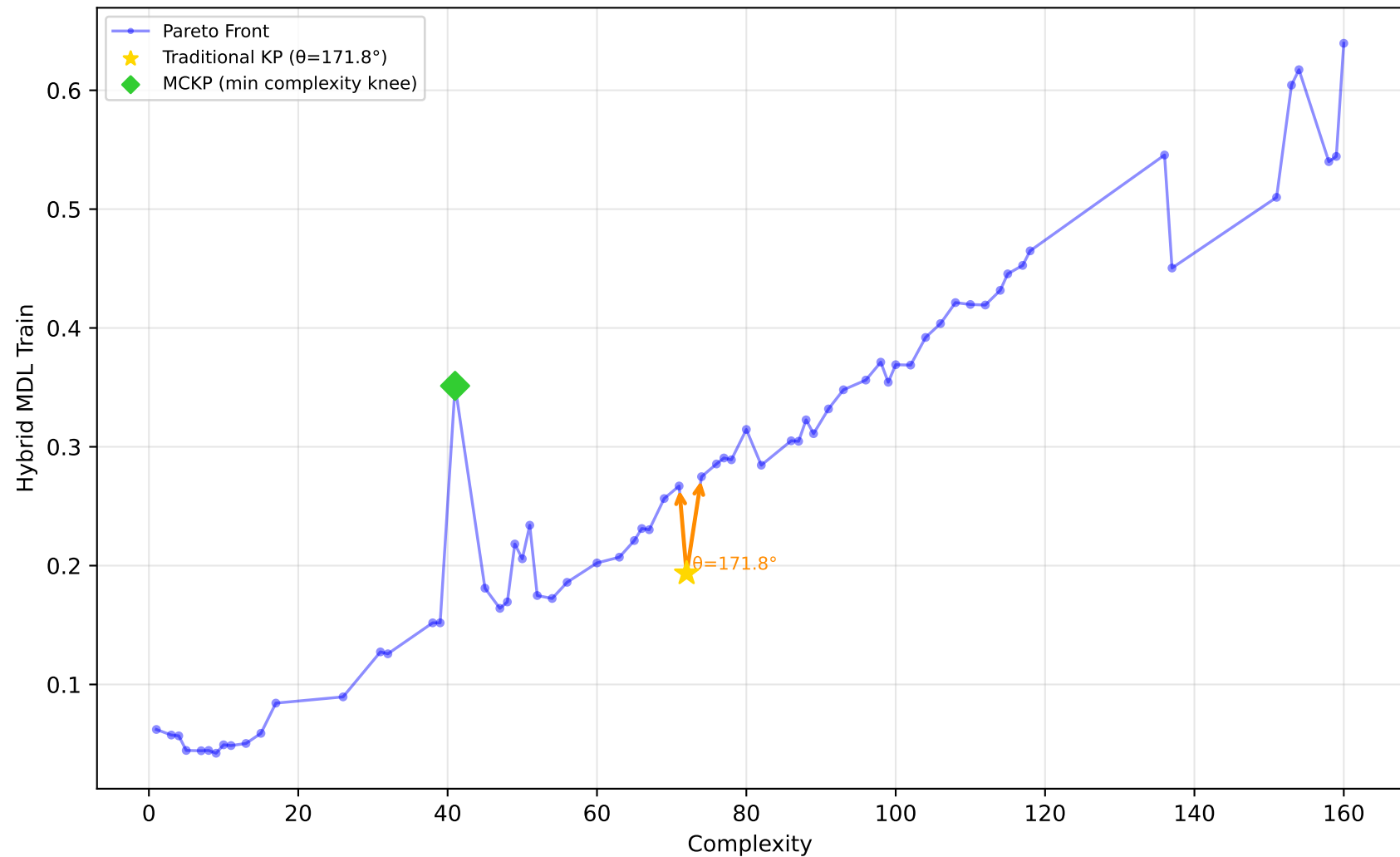
1096_FacultySalaries - Run 2 - SVP - Hybrid MDL Train \lambda_1=0.00, \lambda_2=0.90, \lambda_3=0.00 | Difficulty: 0.52 | Method: mckp
