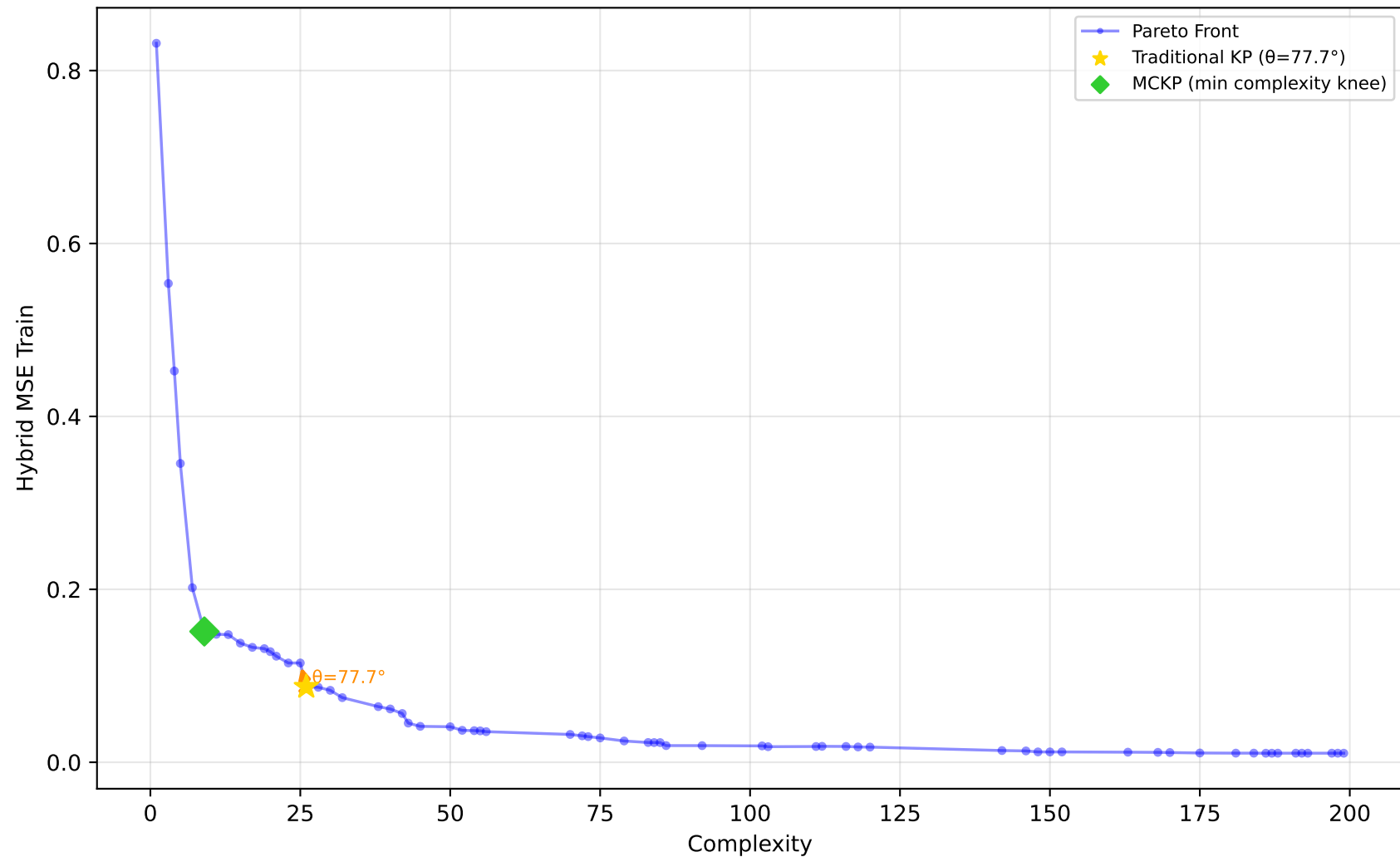
1096_FacultySalaries - Run 30 - MVP - Hybrid MSE Train \lambda_1=0.10, \lambda_2=0.00, \lambda_3=0.00 | Difficulty: 1.00 | Method: hmr
