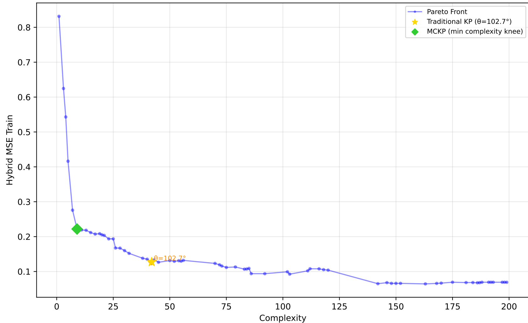
1096_FacultySalaries - Run 30 - MVP - Hybrid MSE Train \lambda_1=1.00, \lambda_2=0.00, \lambda_3=0.00 | Difficulty: 1.00 | Method: hmr
