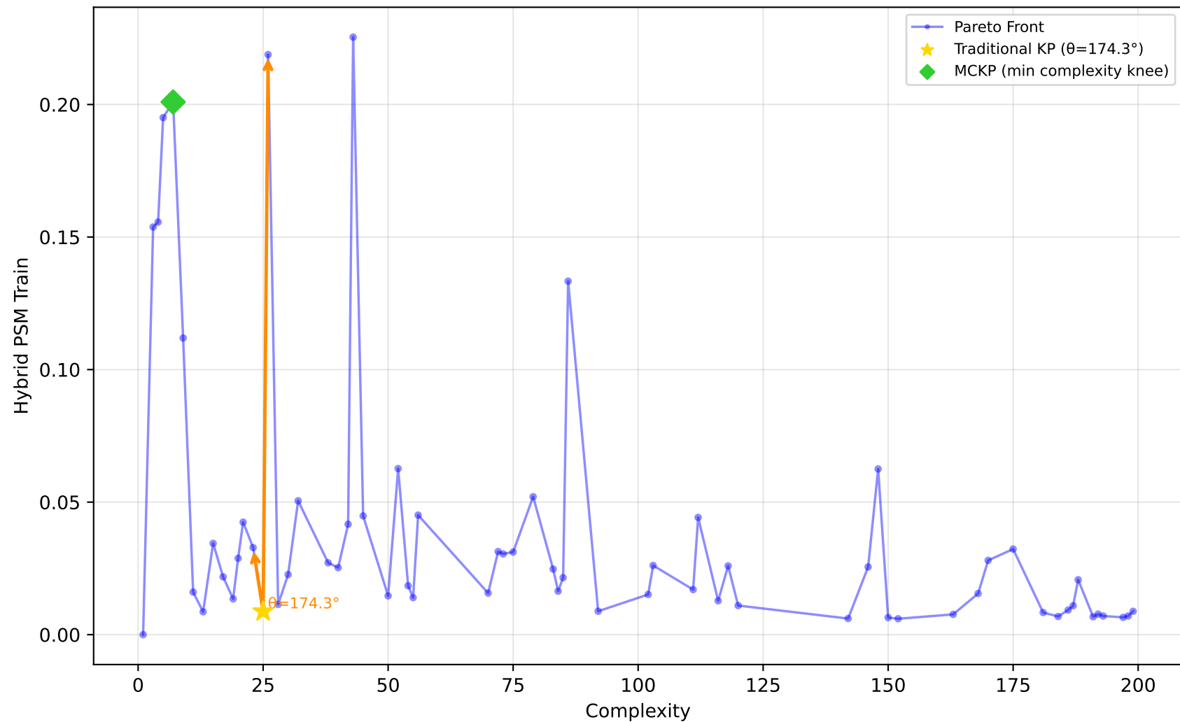
1096_FacultySalaries - Run 30 - MVP - Hybrid PSM Train \lambda_1=0.10, \lambda_2=0.00, \lambda_3=0.00 | Difficulty: 1.00 | Method: hmr
