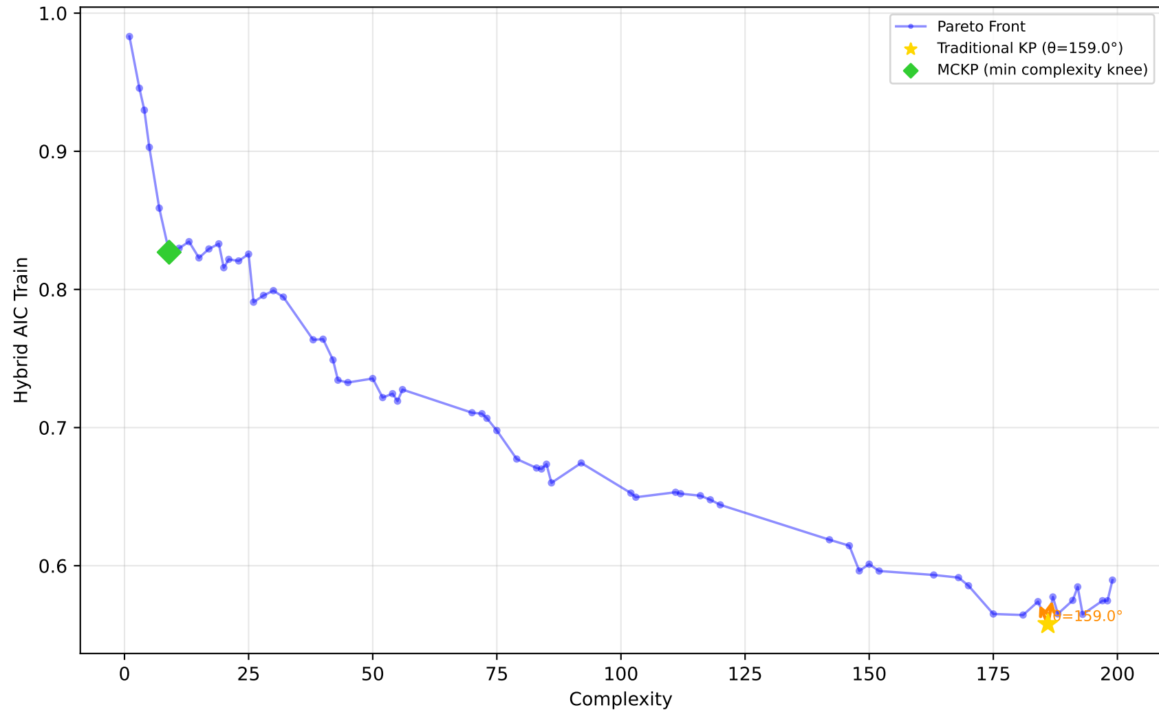
1096_FacultySalaries - Run 30 - SVP - Hybrid AIC Train \lambda_1=0.00, \lambda_2=0.90, \lambda_3=0.00 | Difficulty: 1.00 | Method: hmr
