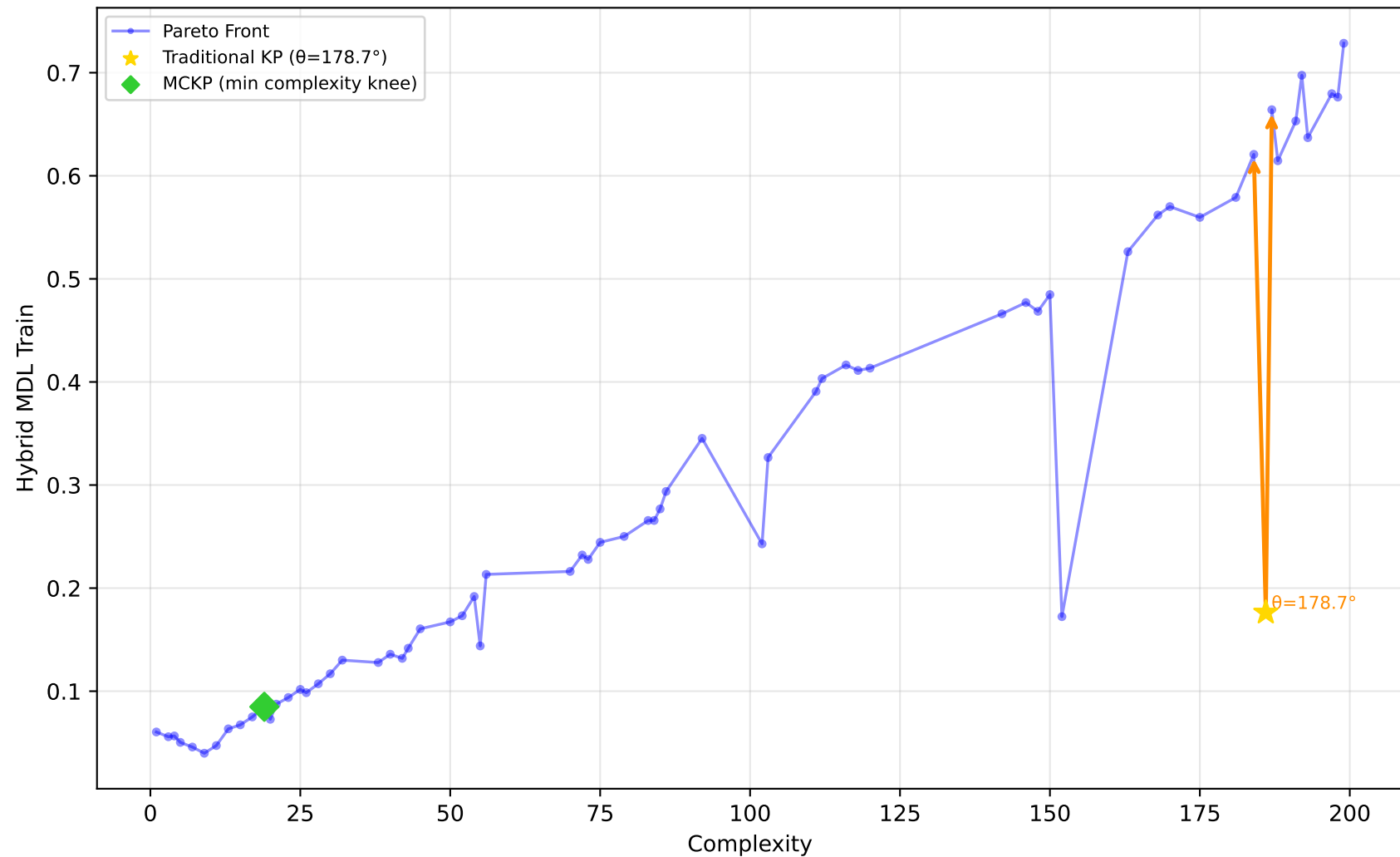
1096_FacultySalaries - Run 30 - SVP - Hybrid MDL Train \lambda_1=0.00, \lambda_2=0.90, \lambda_3=0.00 | Difficulty: 1.00 | Method: hmr
