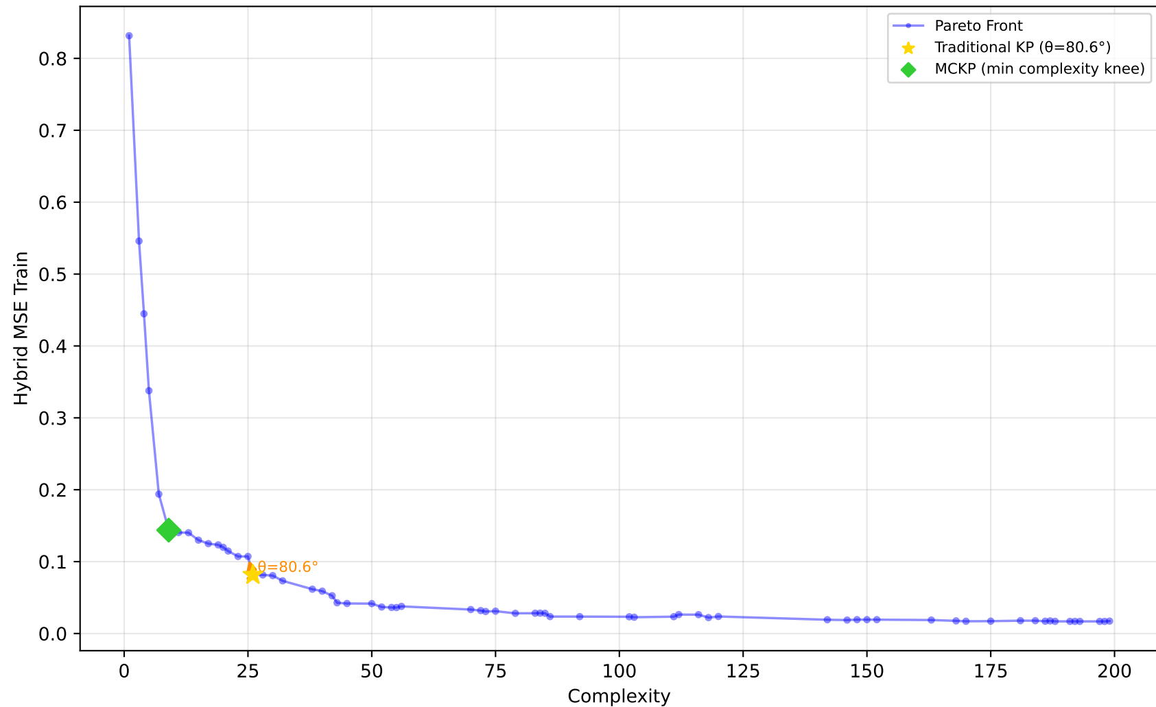
1096_FacultySalaries - Run 30 - SVP - Hybrid MSE Train \lambda_1=0.00 , \lambda_2=0.90 , \lambda_3=0.00 | Difficulty: 1.00 | Method: hmr
