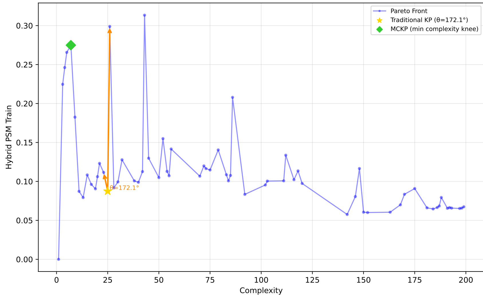
1096_FacultySalaries - Run 30 - SVP - Hybrid PSM Train \lambda_1=1.00 , \lambda_2=0.00 , \lambda_3=0.00 | Difficulty: 1.00 | Method: hmr
