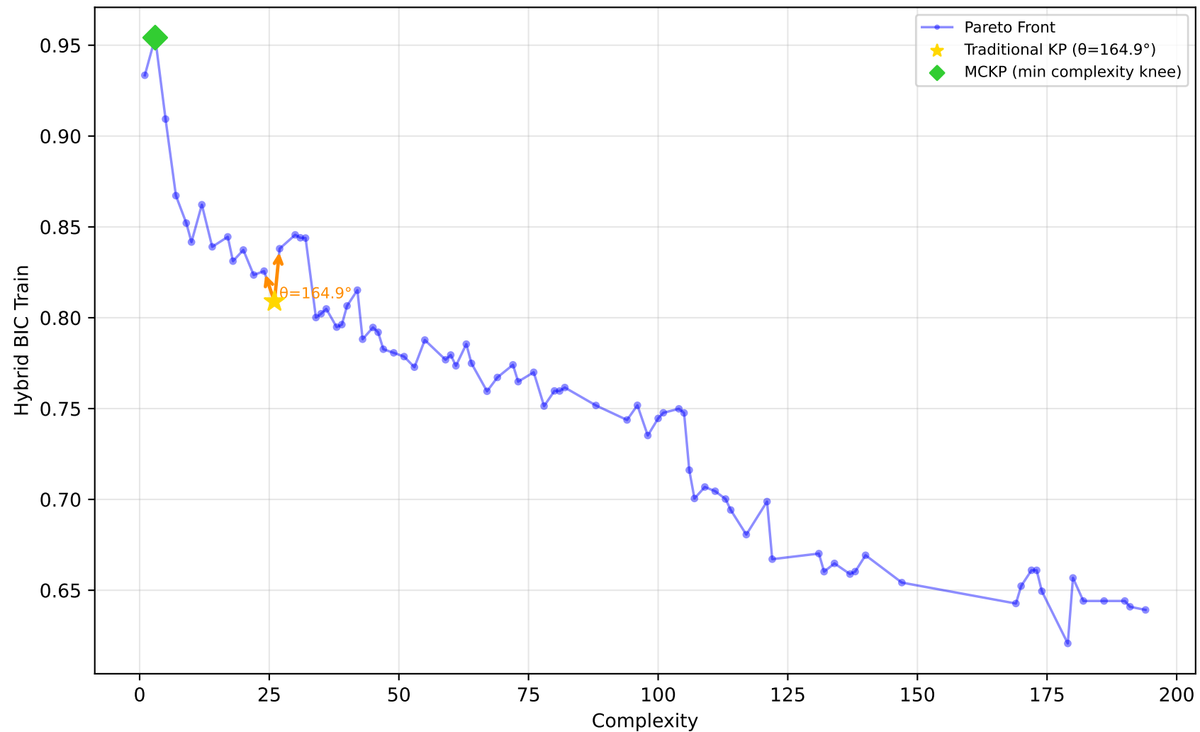
1096_FacultySalaries - Run 3 - MVP - Hybrid BIC Train \lambda_1=1.00 , \lambda_2=0.00 , \lambda_3=0.00 | Difficulty: 1.00 | Method: hmr
