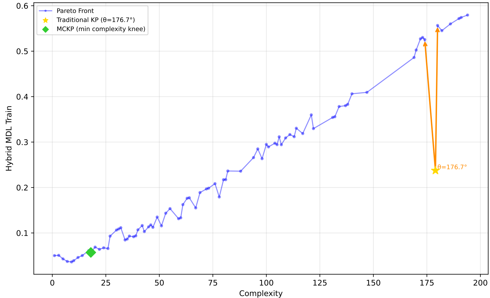
1096_FacultySalaries - Run 3 - MVP - Hybrid MDL Train \lambda_1=0.10, \lambda_2=0.00, \lambda_3=0.00 | Difficulty: 1.00 | Method: hmr
