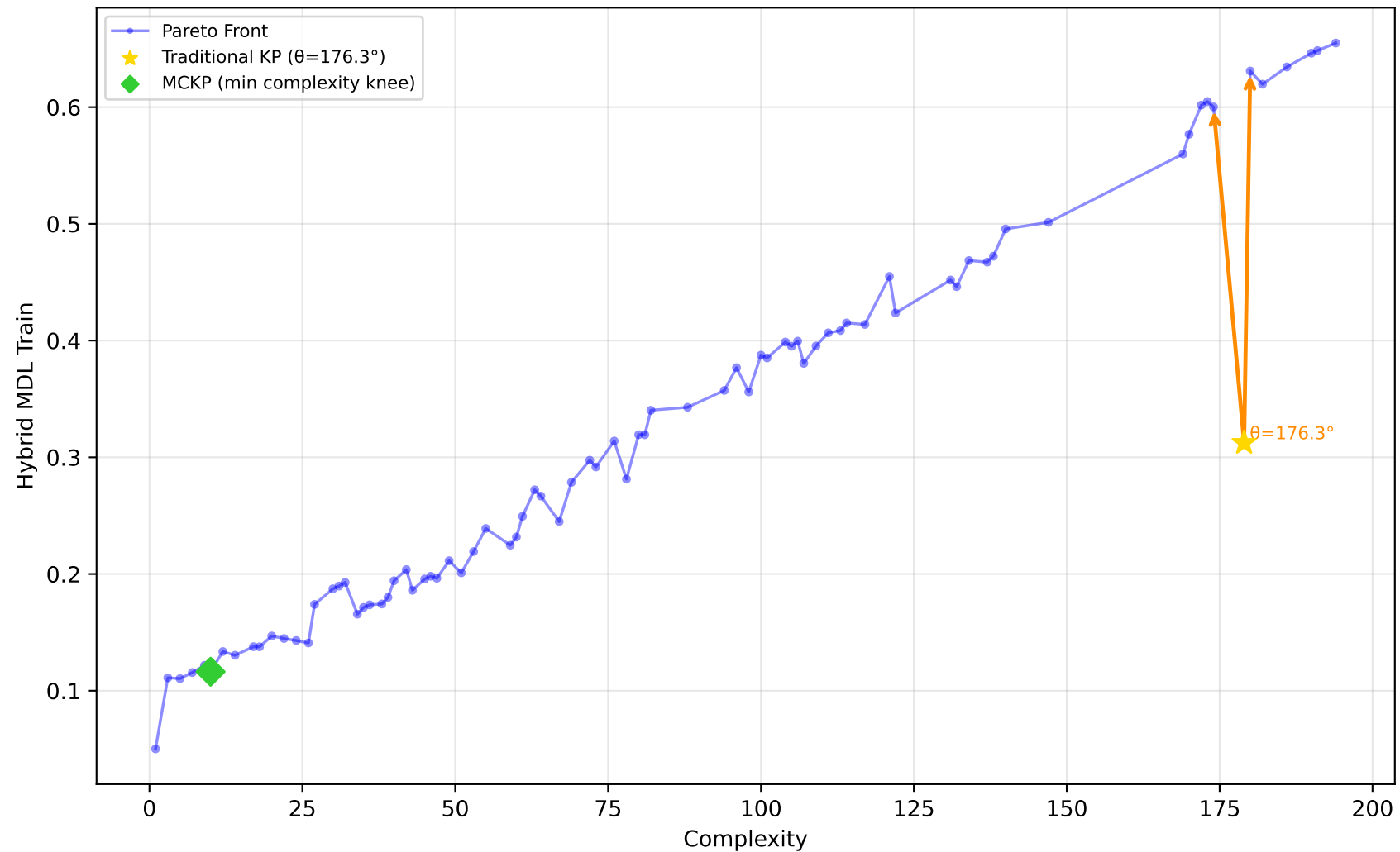
1096_FacultySalaries - Run 3 - MVP - Hybrid MDL Train \lambda_1=1.00 , \lambda_2=0.00 , \lambda_3=0.00 | Difficulty: 1.00 | Method: hmr
