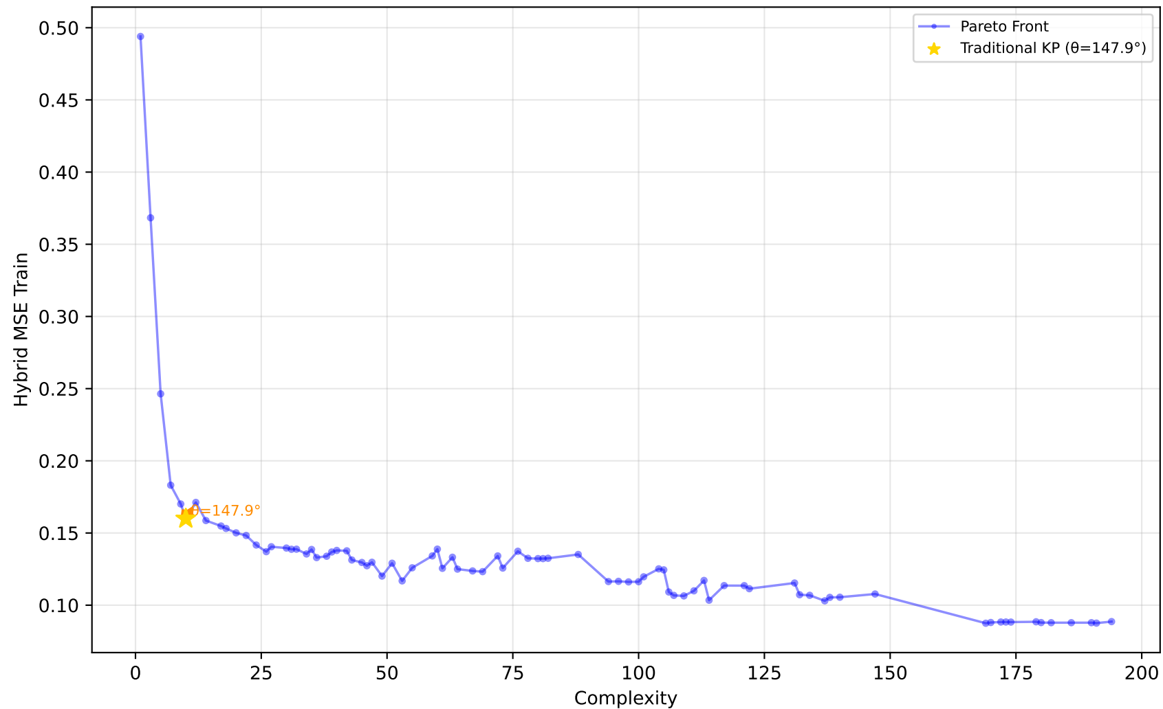
1096_FacultySalaries - Run 3 - MVP - Hybrid MSE Train \lambda_1=1.00 , \lambda_2=0.00 , \lambda_3=0.00 | Difficulty: 1.00 | Method: hmr
