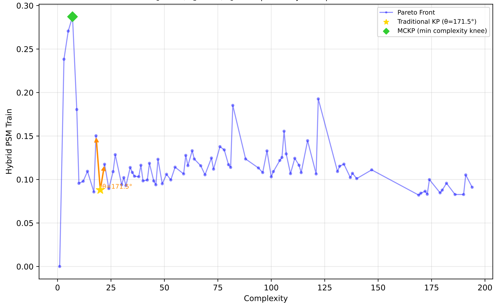
1096_FacultySalaries - Run 3 - MVP - Hybrid PSM Train \lambda_1=1.00 , \lambda_2=0.00 , \lambda_3=0.00 | Difficulty: 1.00 | Method: hmr
