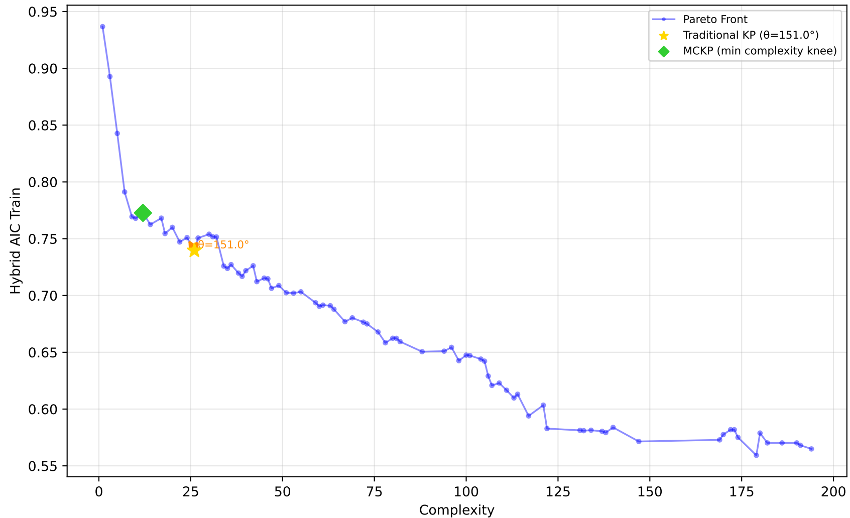
1096_FacultySalaries - Run 3 - SVP - Hybrid AIC Train \lambda_1=0.00, \lambda_2=0.90, \lambda_3=0.00 | Difficulty: 1.00 | Method: hmr
