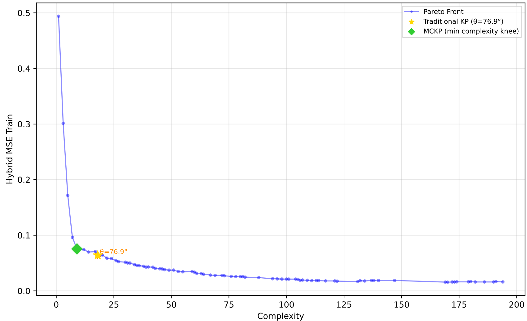
1096_FacultySalaries - Run 3 - SVP - Hybrid MSE Train \lambda_1=0.00, \lambda_2=0.90, \lambda_3=0.00 | Difficulty: 1.00 | Method: hmr
