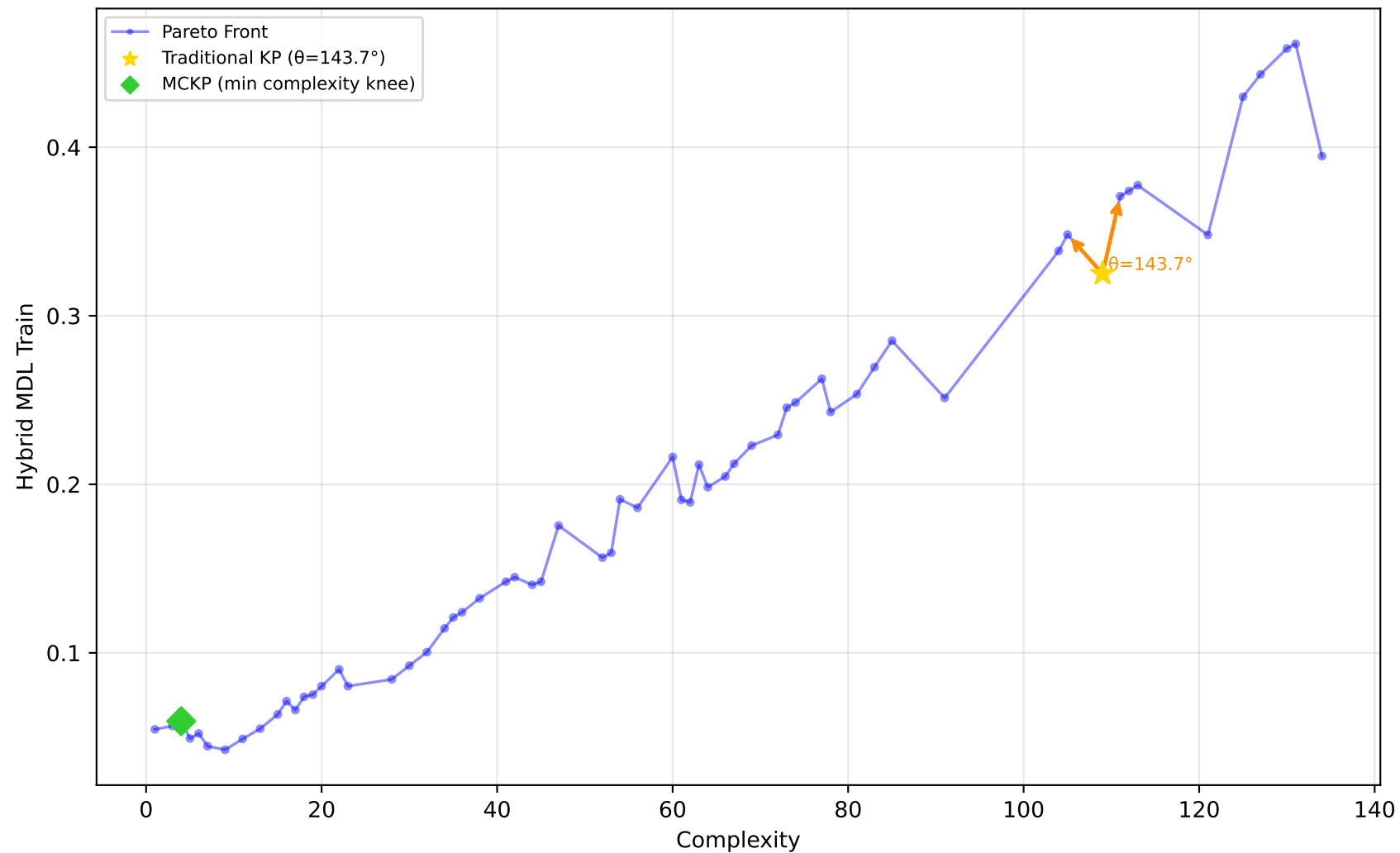
1096_FacultySalaries - Run 4 - MVP - Hybrid MDL Train \lambda_1=0.10, \lambda_2=0.00, \lambda_3=0.00 | Difficulty: 0.50 | Method: mckp
