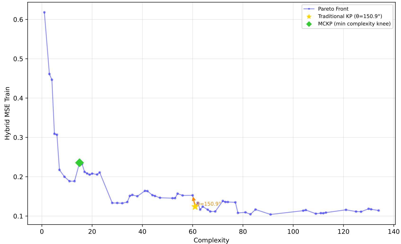
1096_FacultySalaries - Run 4 - MVP - Hybrid MSE Train \lambda_1=1.00, \lambda_2=0.00, \lambda_3=0.00 | Difficulty: 0.50 | Method: mckp
