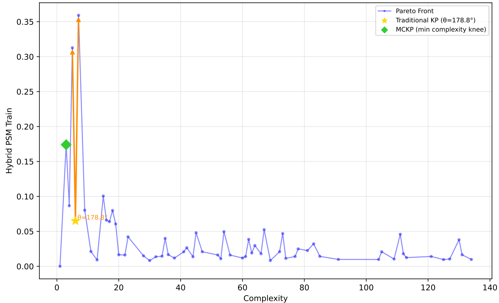
1096_FacultySalaries - Run 4 - MVP - Hybrid PSM Train \lambda_1=0.10, \lambda_2=0.00, \lambda_3=0.00 | Difficulty: 0.50 | Method: mckp
