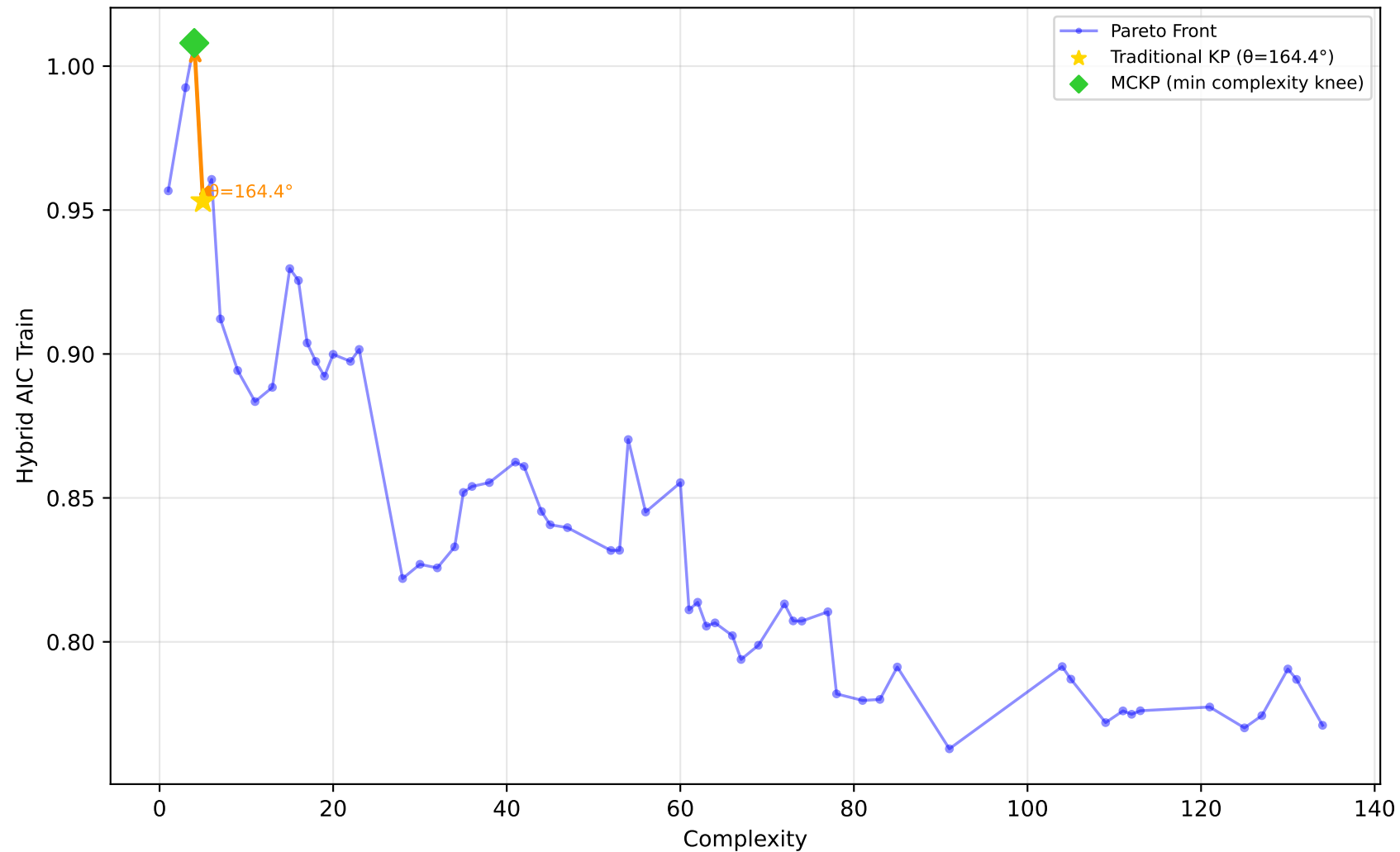
1096_FacultySalaries - Run 4 - SVP - Hybrid AIC Train \lambda_1=1.00, \lambda_2=0.00, \lambda_3=0.00 | Difficulty: 0.50 | Method: mckp
