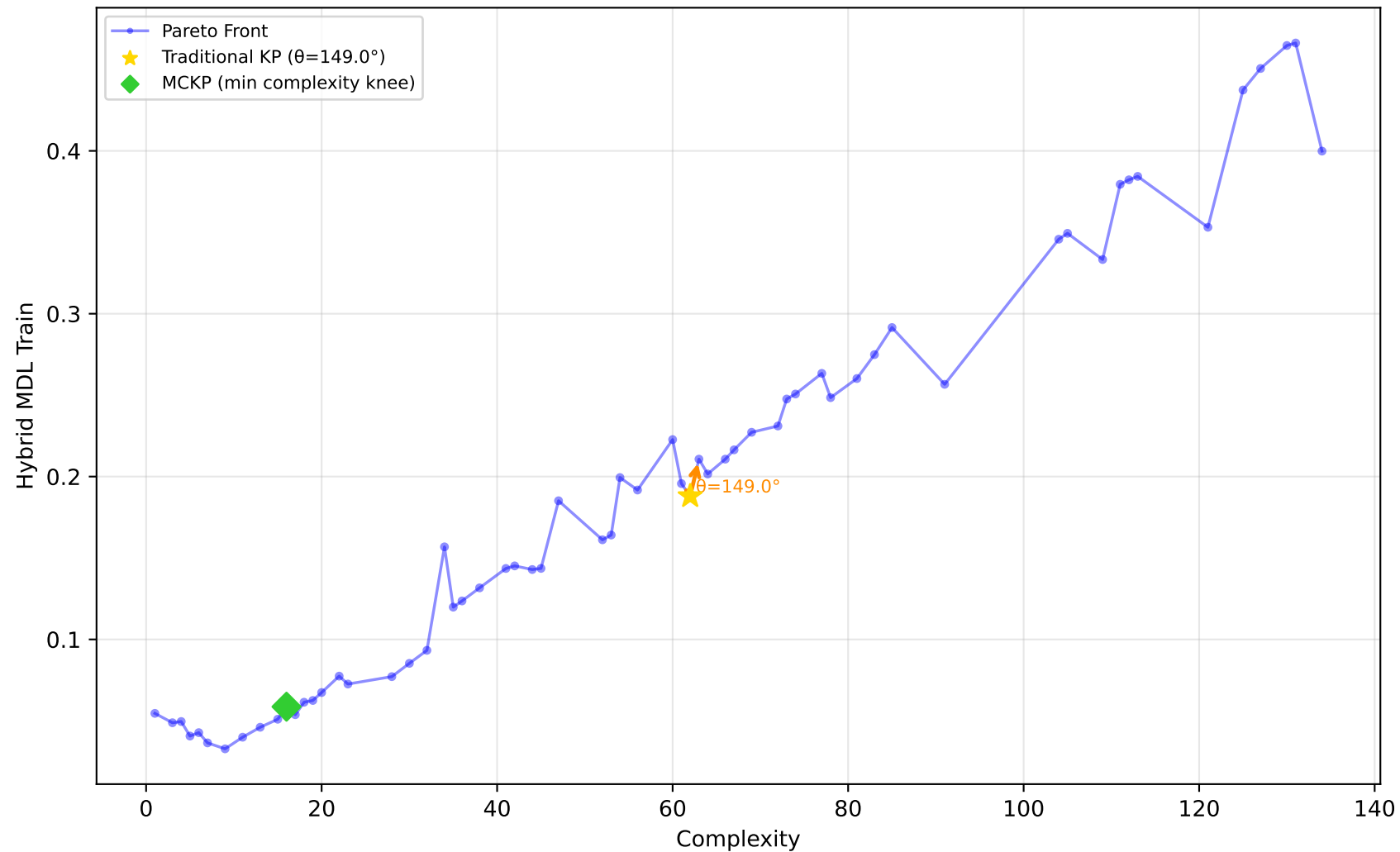
1096_FacultySalaries - Run 4 - SVP - Hybrid MDL Train \lambda_1=0.00, \lambda_2=0.90, \lambda_3=0.00 | Difficulty: 0.50 | Method: mckp
