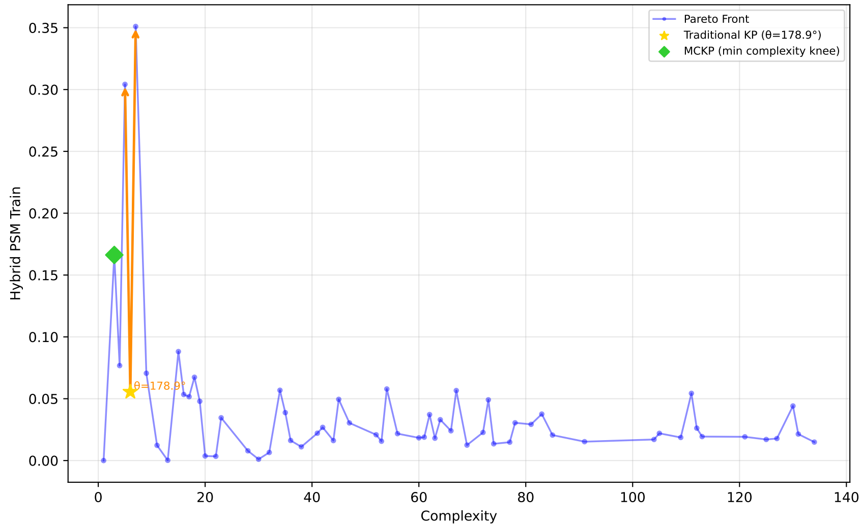
1096_FacultySalaries - Run 4 - SVP - Hybrid PSM Train \lambda_1=0.00, \lambda_2=0.90, \lambda_3=0.00 | Difficulty: 0.50 | Method: mckp
