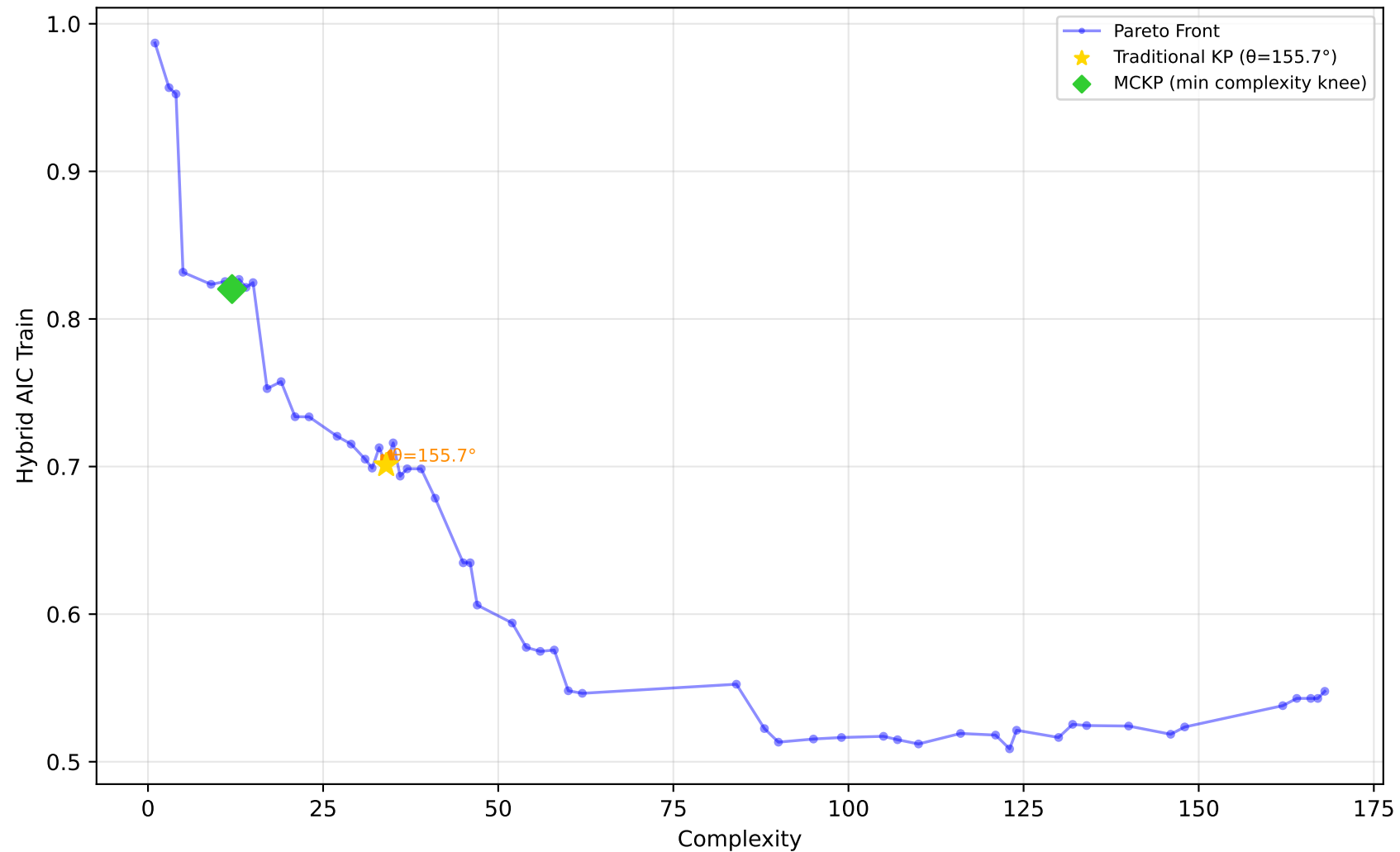
1096_FacultySalaries - Run 5 - MVP - Hybrid AIC Train \lambda_1=0.10, \lambda_2=0.00, \lambda_3=0.00 | Difficulty: 0.11 | Method: mckp
