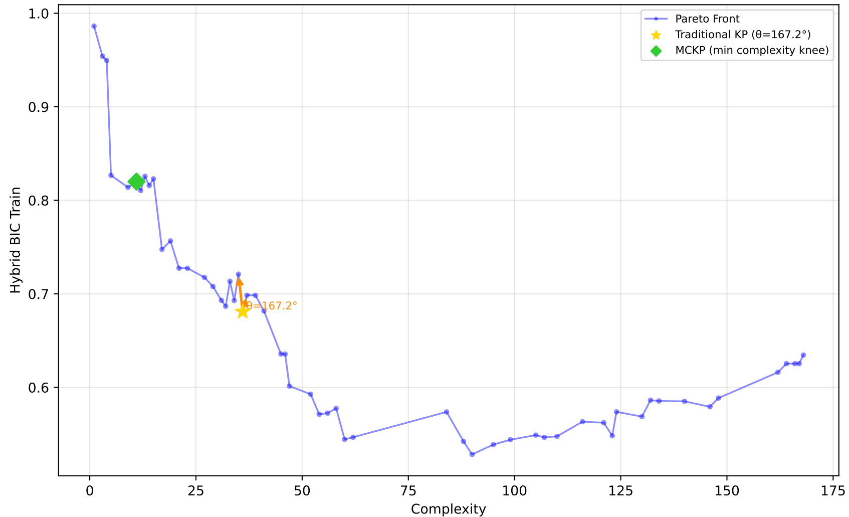
1096_FacultySalaries - Run 5 - MVP - Hybrid BIC Train \lambda_1=0.10, \lambda_2=0.00, \lambda_3=0.00 | Difficulty: 0.11 | Method: mckp
