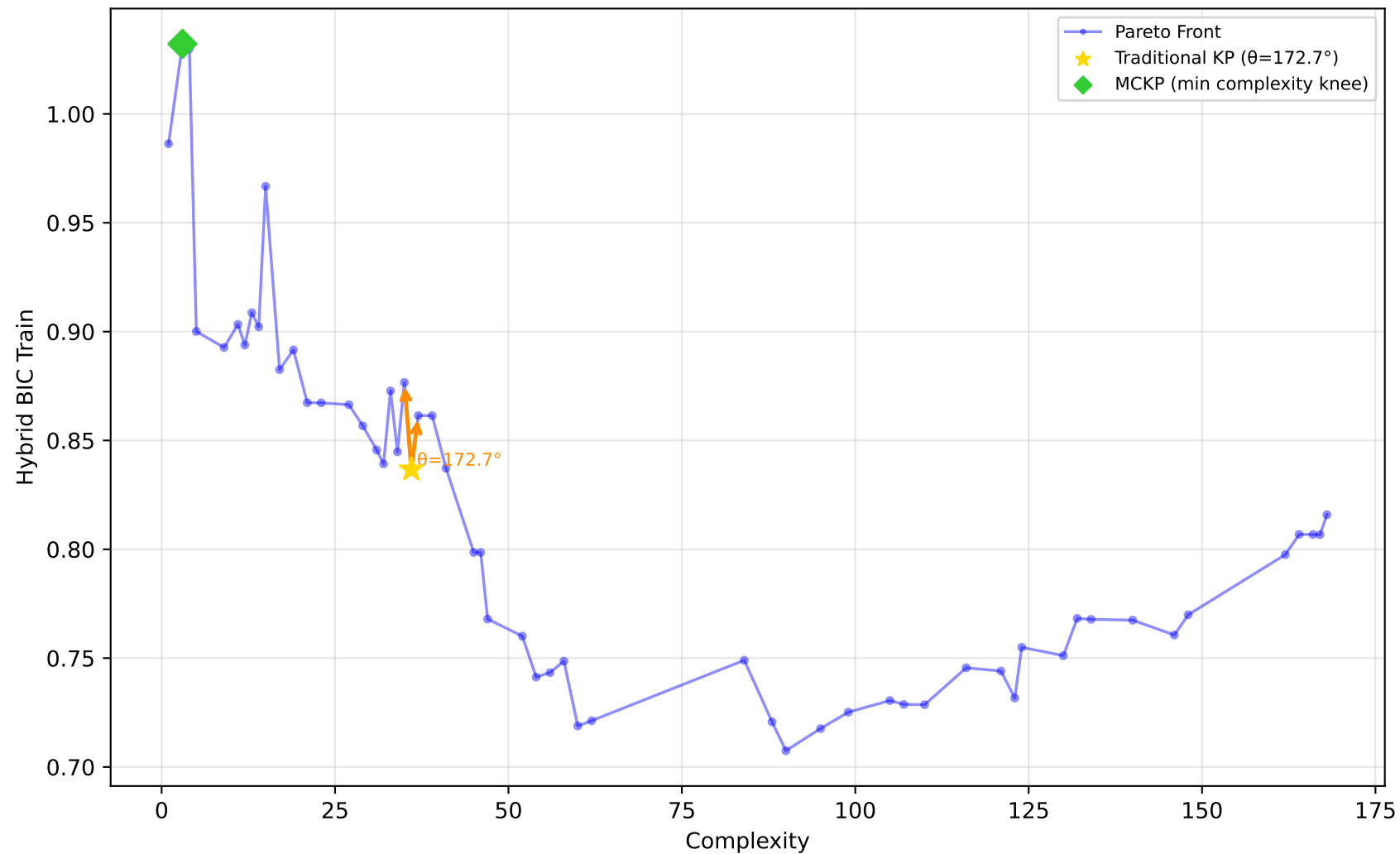
1096_FacultySalaries - Run 5 - MVP - Hybrid BIC Train \lambda_1=1.00, \lambda_2=0.00, \lambda_3=0.00 | Difficulty: 0.11 | Method: mckp
