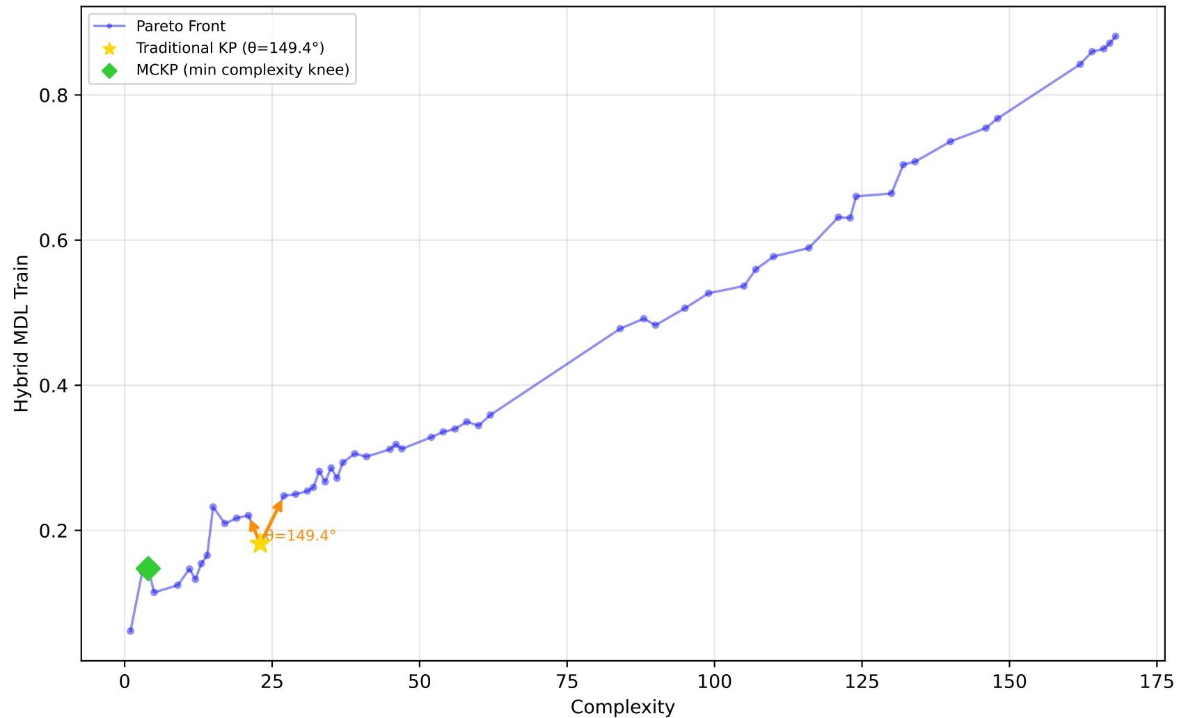
1096_FacultySalaries - Run 5 - MVP - Hybrid MDL Train \lambda_1=1.00, \lambda_2=0.00, \lambda_3=0.00 | Difficulty: 0.11 | Method: mckp
