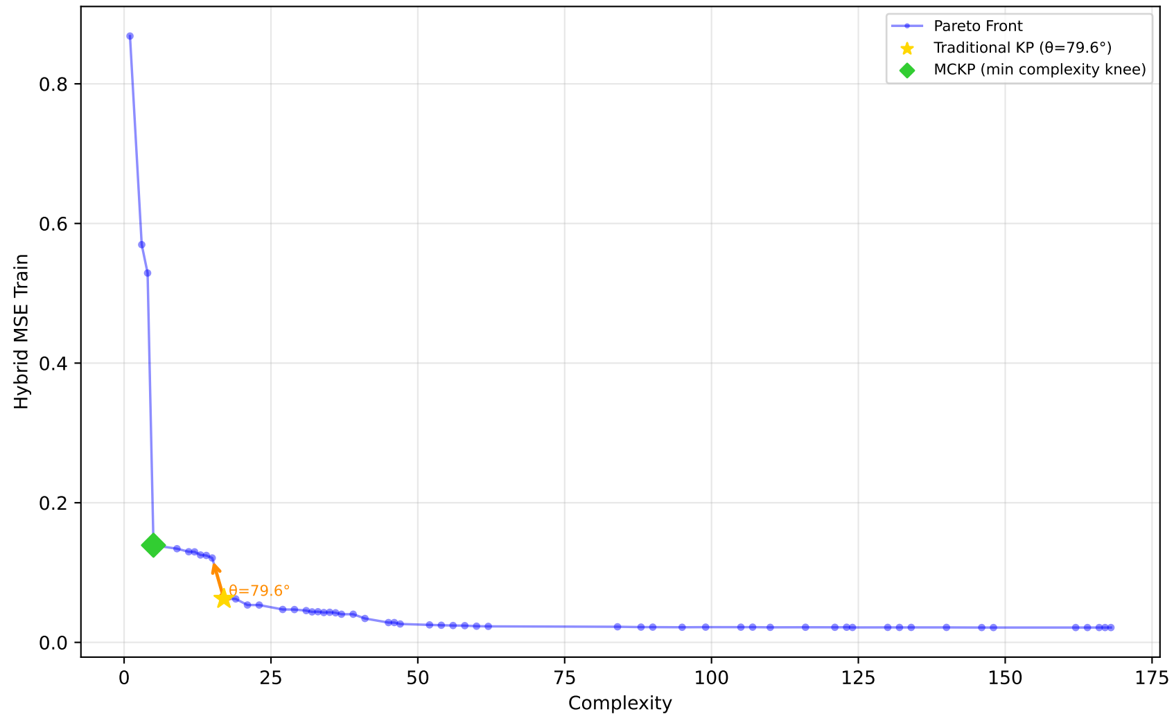
1096_FacultySalaries - Run 5 - MVP - Hybrid MSE Train \lambda_1=0.10, \lambda_2=0.00, \lambda_3=0.00 | Difficulty: 0.11 | Method: mckp
