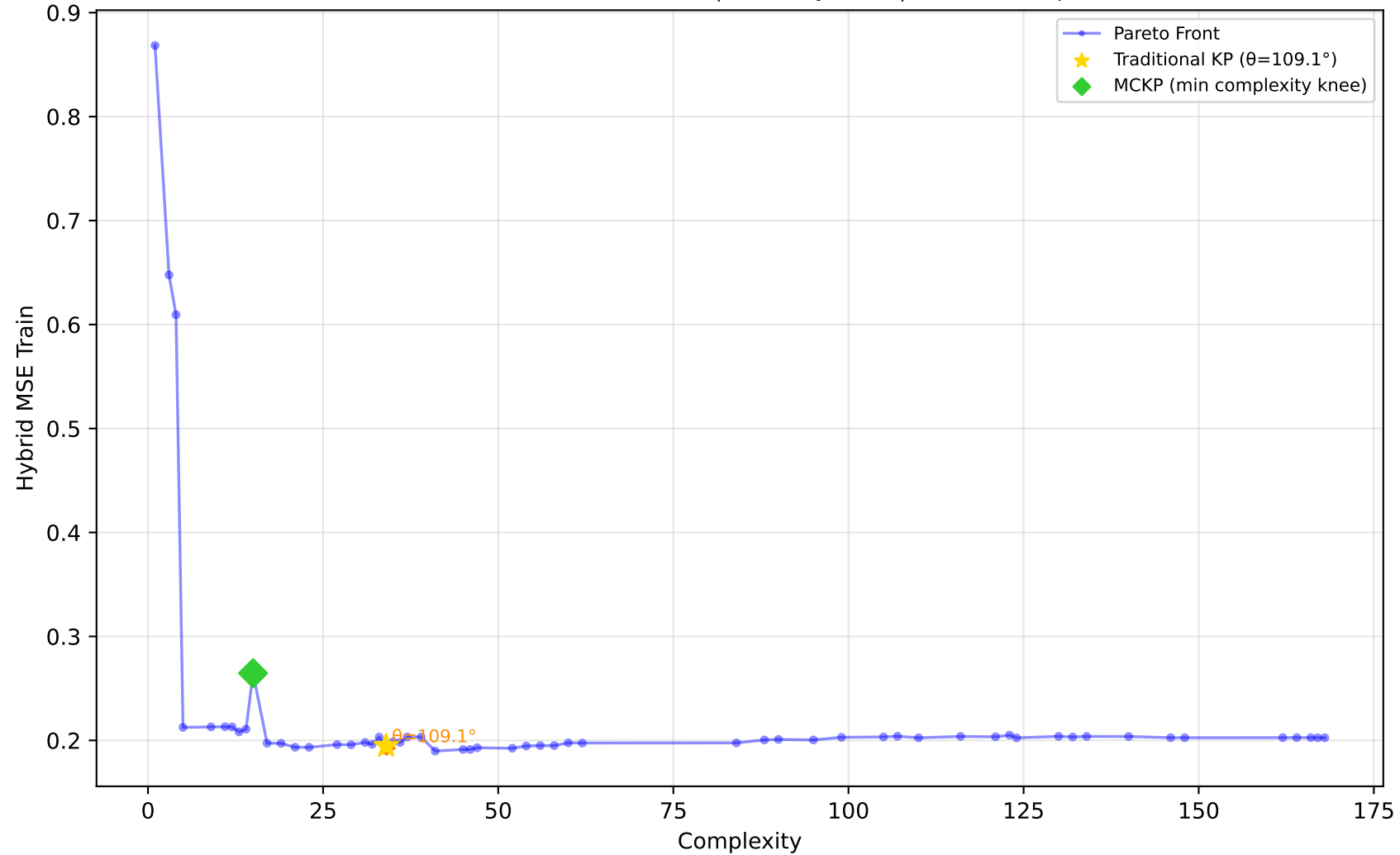
1096_FacultySalaries - Run 5 - MVP - Hybrid MSE Train \lambda_1=1.00, \lambda_2=0.00, \lambda_3=0.00 | Difficulty: 0.11 | Method: mckp
