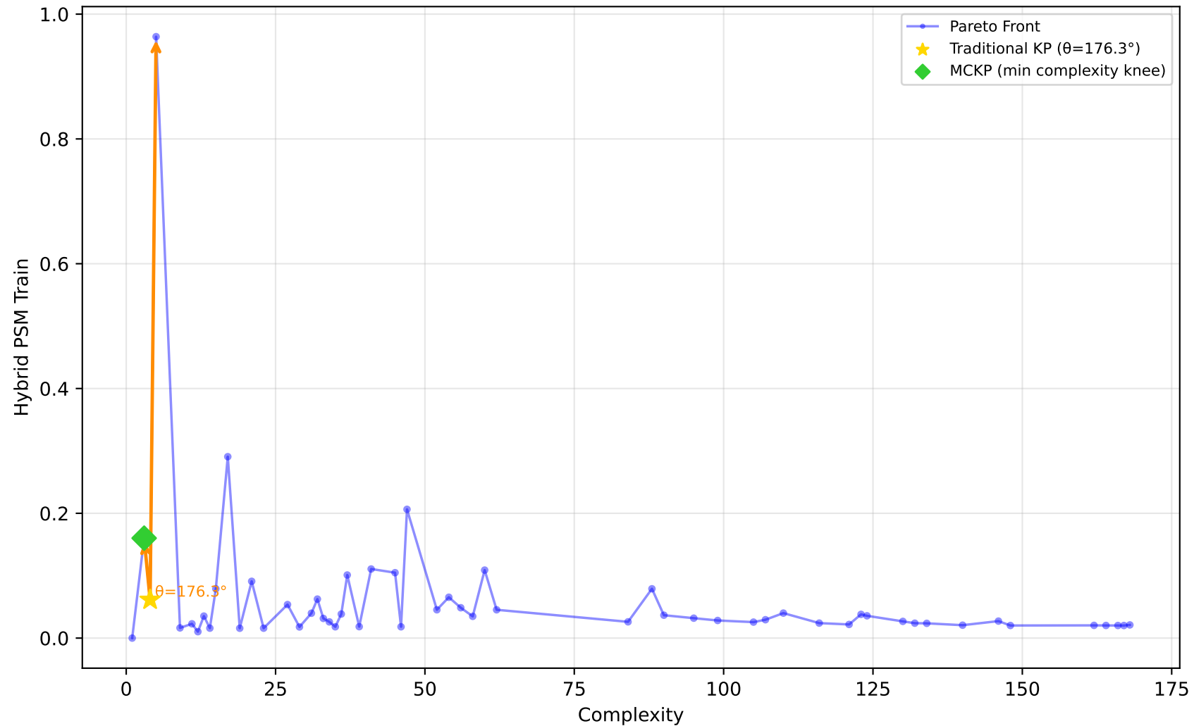
1096_FacultySalaries - Run 5 - MVP - Hybrid PSM Train \lambda_1=0.10, \lambda_2=0.00, \lambda_3=0.00 | Difficulty: 0.11 | Method: mckp
